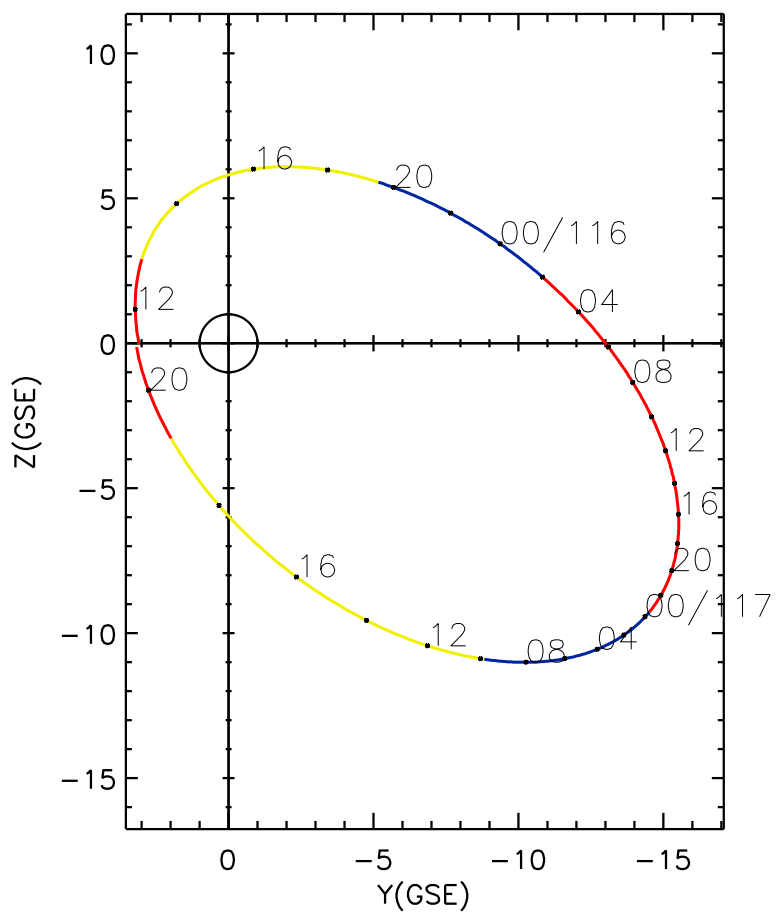
CLUSTER 2 orbit 2006 115 (04/25) 11:31 UT to 2006 117 (04/27) 20:36 UT
