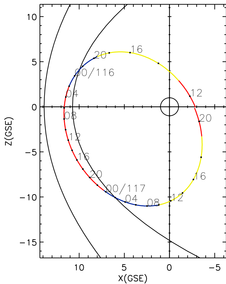
CLUSTER 2 orbit 2006 115 (04/25) 11:31 UT to 2006 117 (04/27) 20:36 UT
