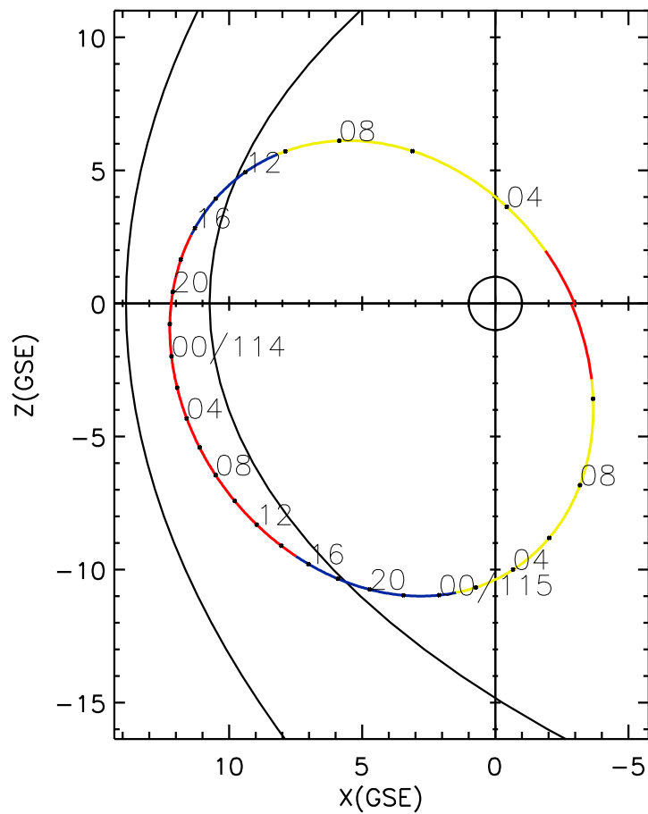
CLUSTER 2 orbit 2006 113 (04/23) 02:21 UT to 2006 115 (04/25) 11:31 UT
