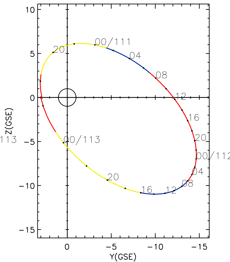
CLUSTER 2 orbit 2006 110 (04/20) 17:11 UT to 2006 113 (04/23) 02:21 UT
