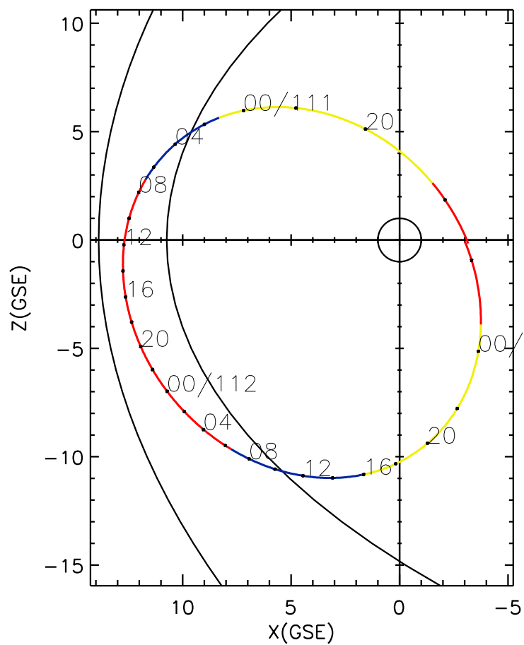
CLUSTER 2 orbit 2006 110 (04/20) 17:11 UT to 2006 113 (04/23) 02:21 UT
