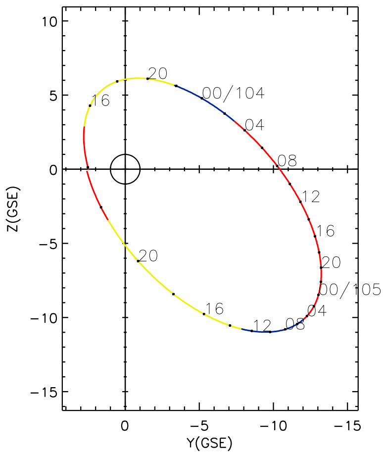
CLUSTER 2 orbit 2006 103 (04/13) 13:56 UT to 2006 105 (04/15) 23:01 UT
