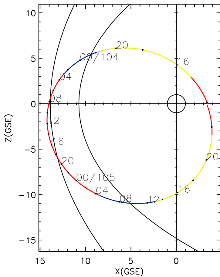
CLUSTER 2 orbit 2006 103 (04/13) 13:56 UT to 2006 105 (04/15) 23:01 UT
