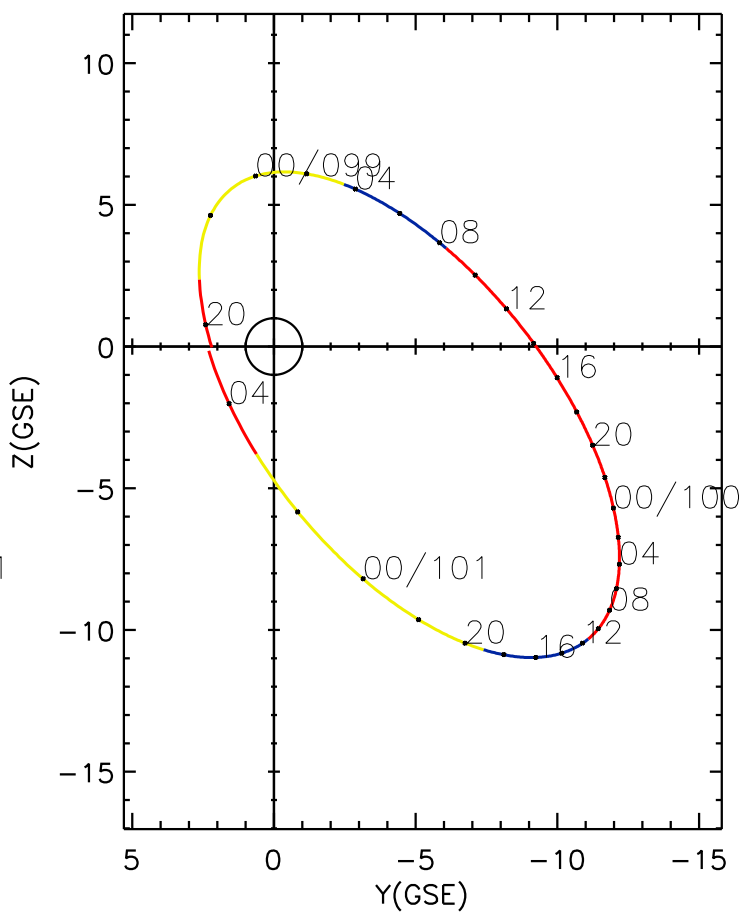
CLUSTER 2 orbit 2006 098 (04/08) 19:41 UT to 2006 101 (04/11) 04:46 UT
