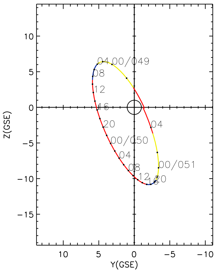
CLUSTER 2 orbit 2006 048 (02/17) 20:01 UT to 2006 051 (02/20) 05:11 UT
