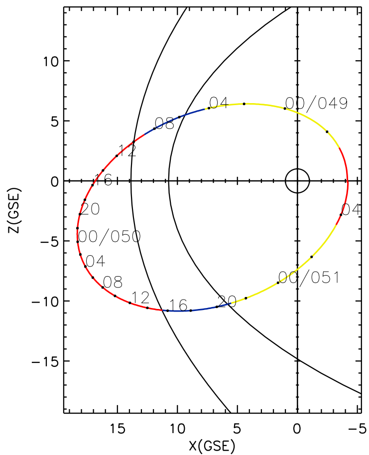
CLUSTER 2 orbit 2006 048 (02/17) 20:01 UT to 2006 051 (02/20) 05:11 UT
