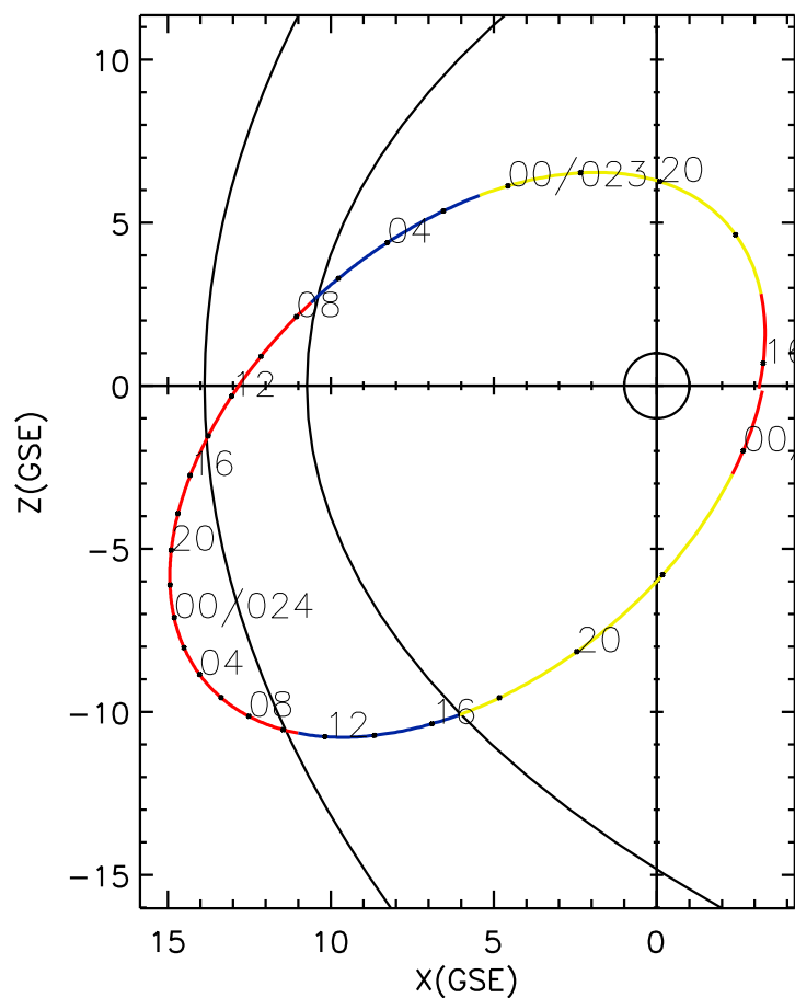
CLUSTER 2 orbit 2006 022 (01/22) 15:41 UT to 2006 025 (01/25) 00:46 UT
