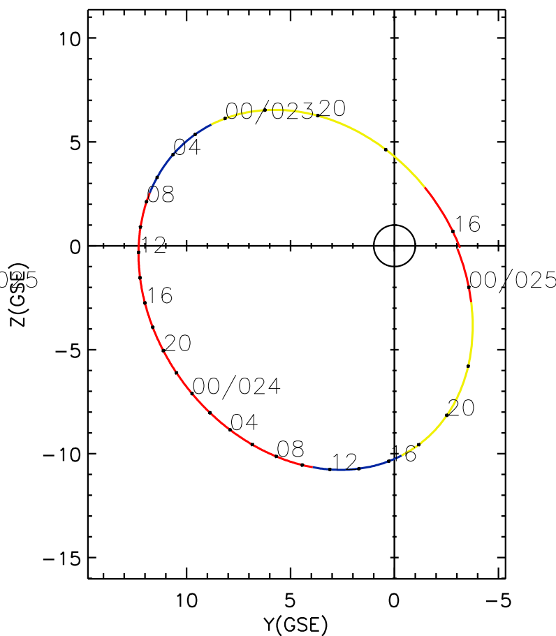
CLUSTER 2 orbit 2006 022 (01/22) 15:41 UT to 2006 025 (01/25) 00:46 UT
