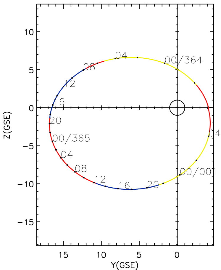
CLUSTER 2 orbit 2005 363 (12/29) 20:31 UT to 2006 001 (01/01) 05:36 UT
