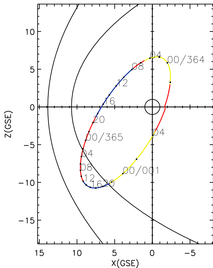
CLUSTER 2 orbit 2005 363 (12/29) 20:31 UT to 2006 001 (01/01) 05:36 UT
