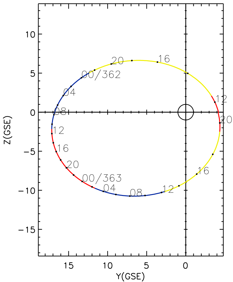
CLUSTER 2 orbit 2005 361 (12/27) 11:26 UT to 2005 363 (12/29) 20:31 UT
