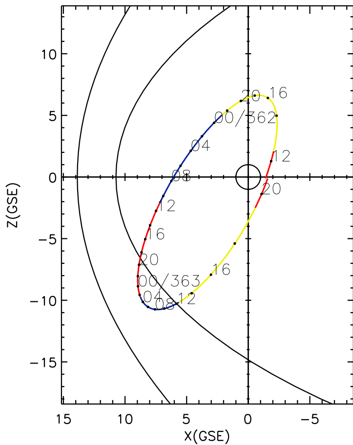
CLUSTER 2 orbit 2005 361 (12/27) 11:26 UT to 2005 363 (12/29) 20:31 UT
