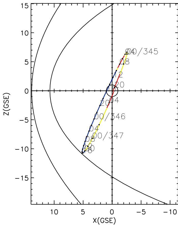
CLUSTER 2 orbit 2005 344 (12/10) 19:41 UT to 2005 347 (12/13) 04:46 UT
