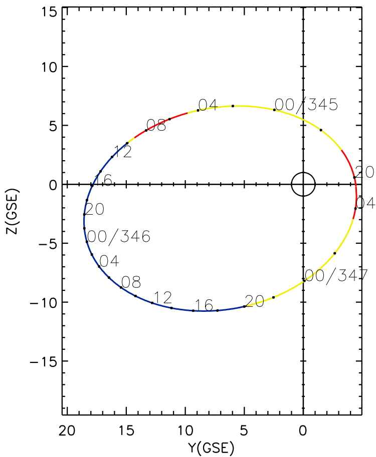
CLUSTER 2 orbit 2005 344 (12/10) 19:41 UT to 2005 347 (12/13) 04:46 UT
