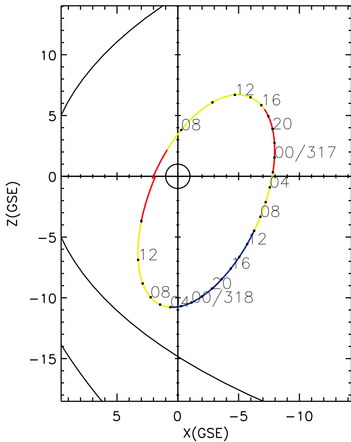
CLUSTER 2 orbit 2005 316 (11/12) 06:11 UT to 2005 318 (11/14) 15:36 UT
