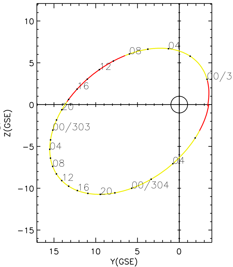
CLUSTER 2 orbit 2005 301 (10/28) 22:36 UT to 2005 304 (10/31) 07:46 UT
