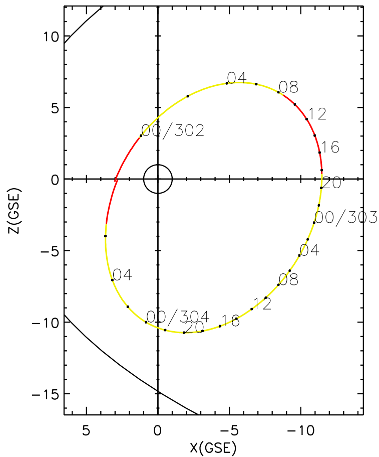
CLUSTER 2 orbit 2005 301 (10/28) 22:36 UT to 2005 304 (10/31) 07:46 UT
