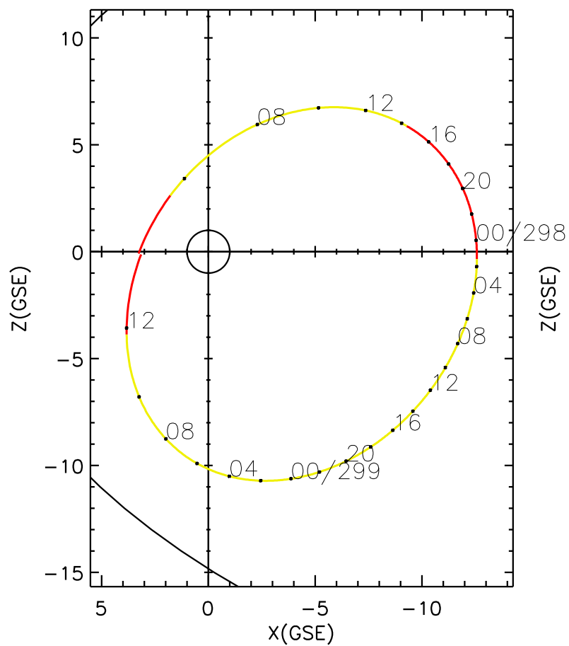
CLUSTER 2 orbit 2005 297 (10/24) 04:26 UT to 2005 299 (10/26) 13:31 UT
