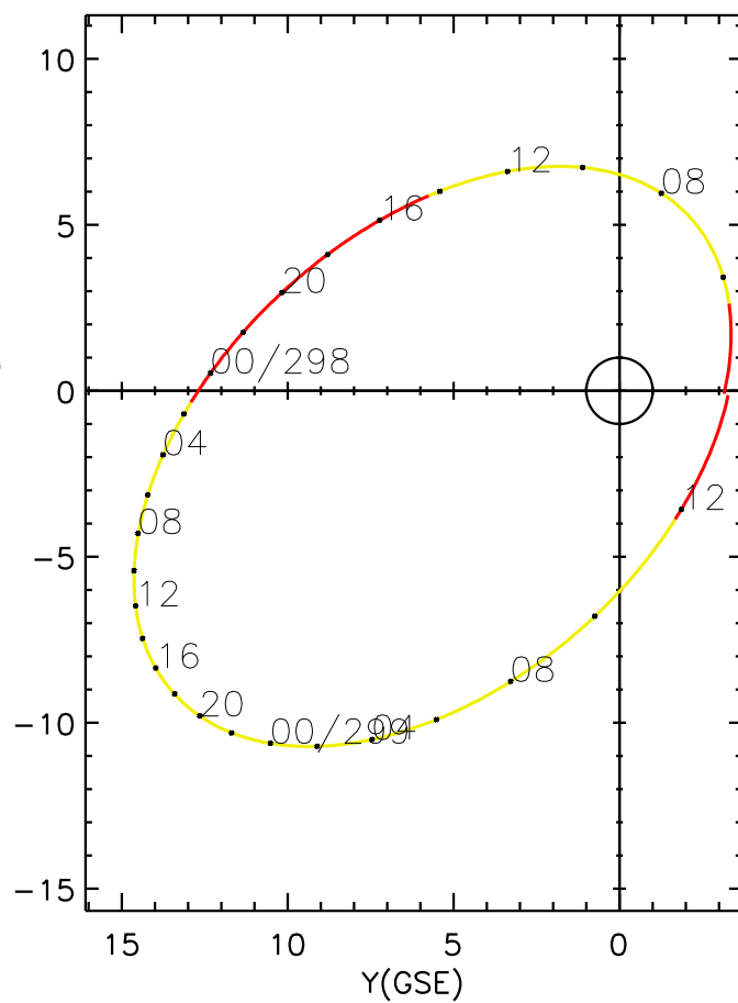
CLUSTER 2 orbit 2005 297 (10/24) 04:26 UT to 2005 299 (10/26) 13:31 UT
