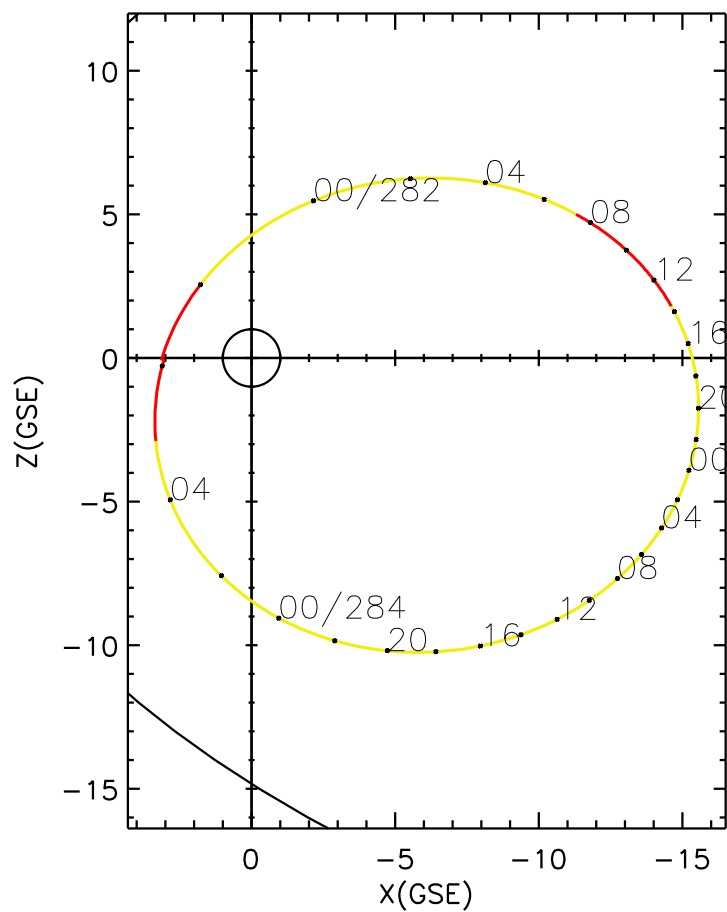
CLUSTER 2 orbit 2005 281 (10/08) 21:00 UT to 2005 284 (10/11) 06:05 UT
