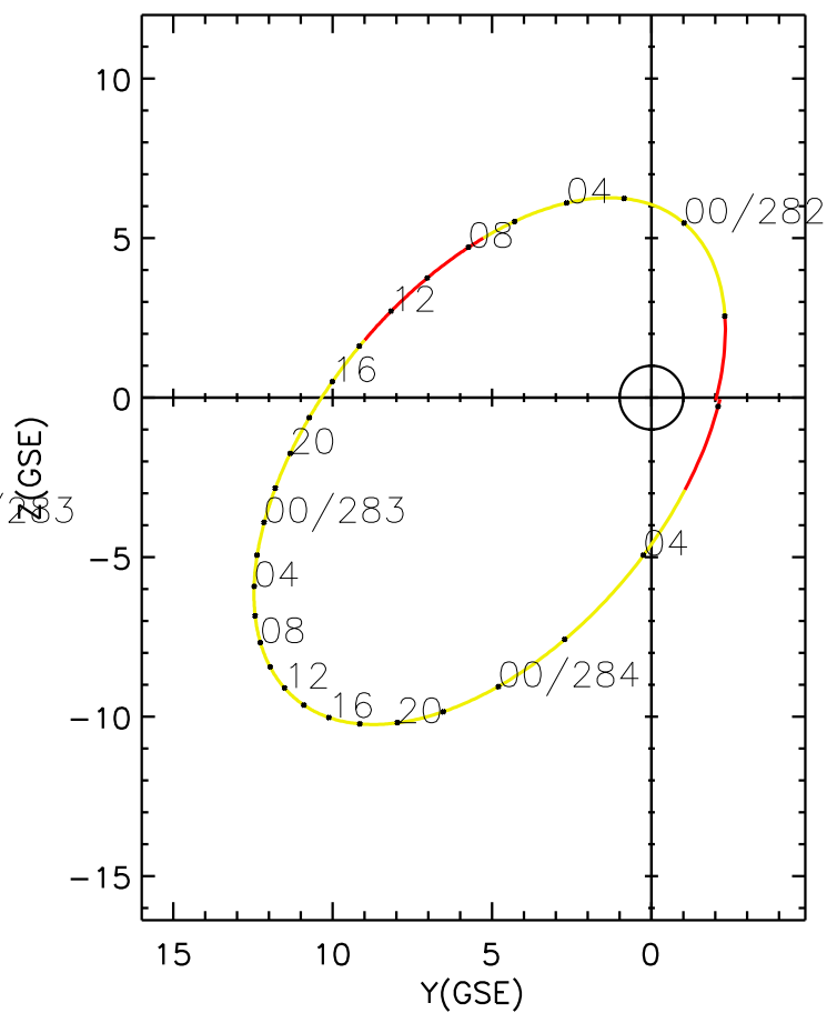
CLUSTER 2 orbit 2005 281 (10/08) 21:00 UT to 2005 284 (10/11) 06:05 UT
