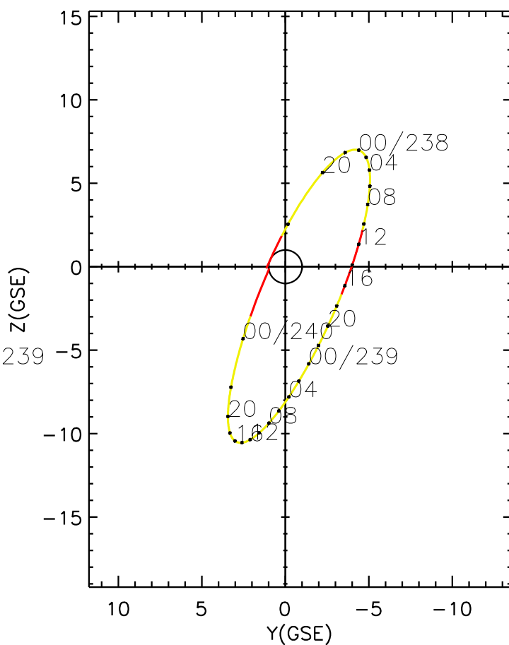
CLUSTER 2 orbit 2005 237 (08/25) 16:51 UT to 2005 240 (08/28) 01:56 UT
