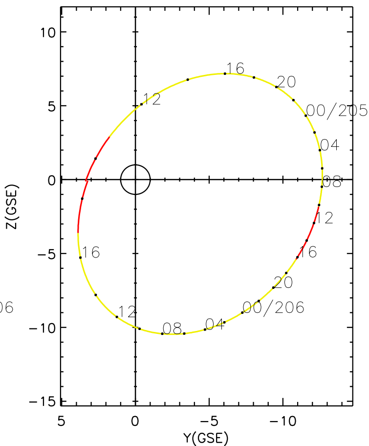
CLUSTER 2 orbit 2005 204 (07/23) 09:21 UT to 2005 206 (07/25) 18:31 UT
