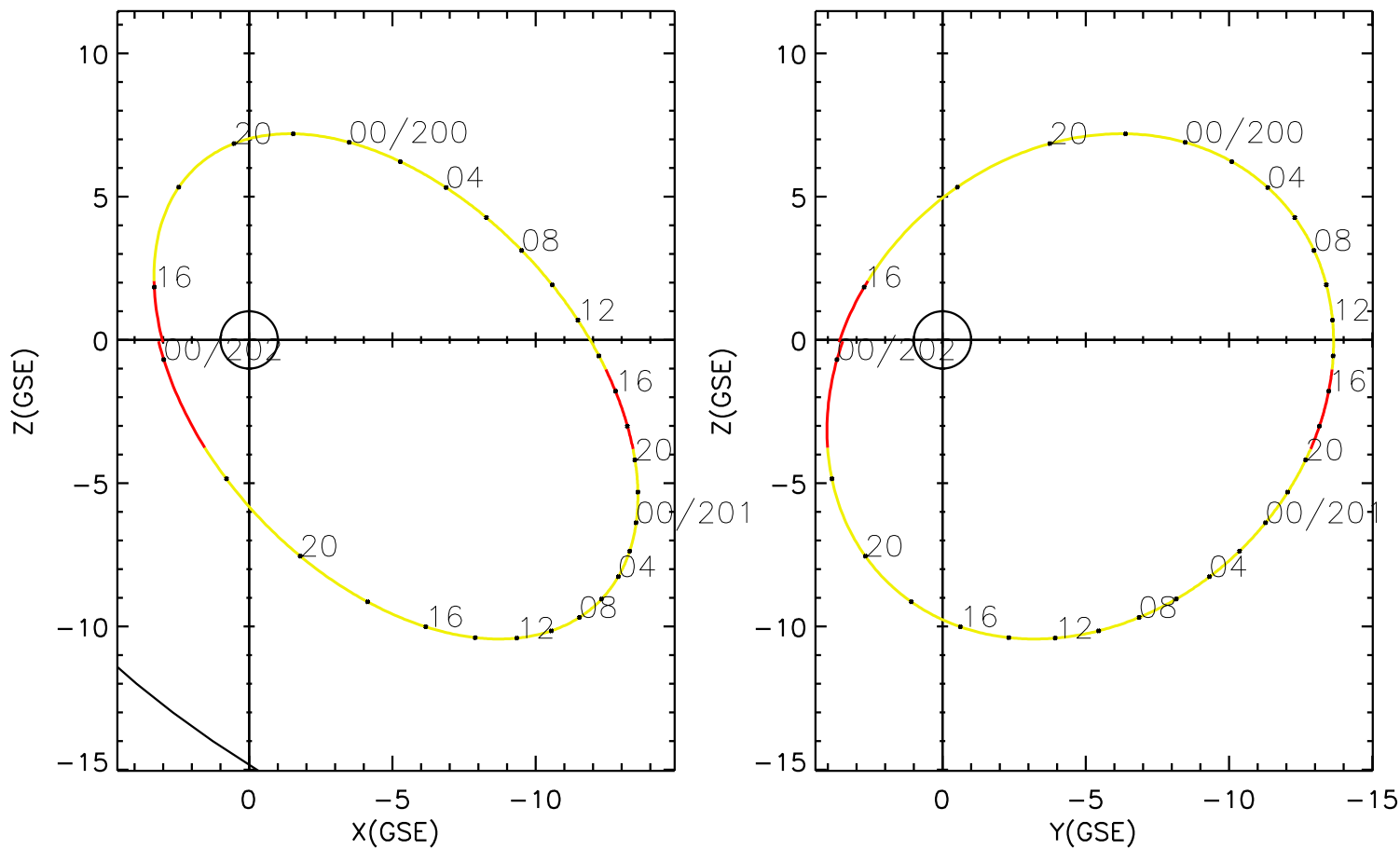
CLUSTER 2 orbit 2005 199 (07/18) 15:11 UT to 2005 202 (07/21) 00:16 UT
