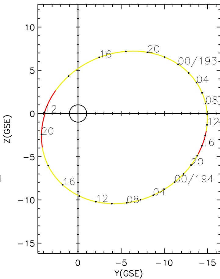
CLUSTER 2 orbit 2005 192 (07/11) 11:56 UT to 2005 194 (07/13) 21:01 UT
