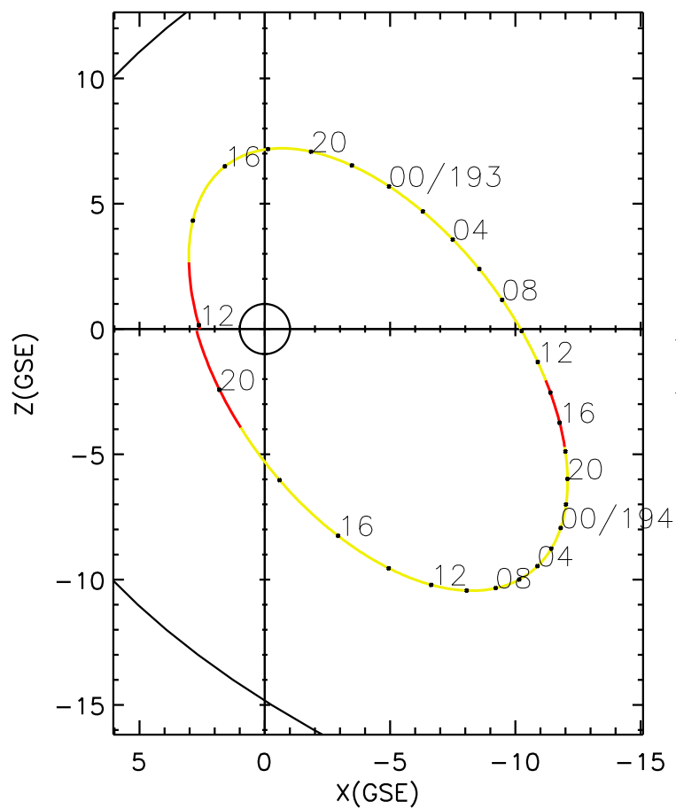
CLUSTER 2 orbit 2005 192 (07/11) 11:56 UT to 2005 194 (07/13) 21:01 UT
