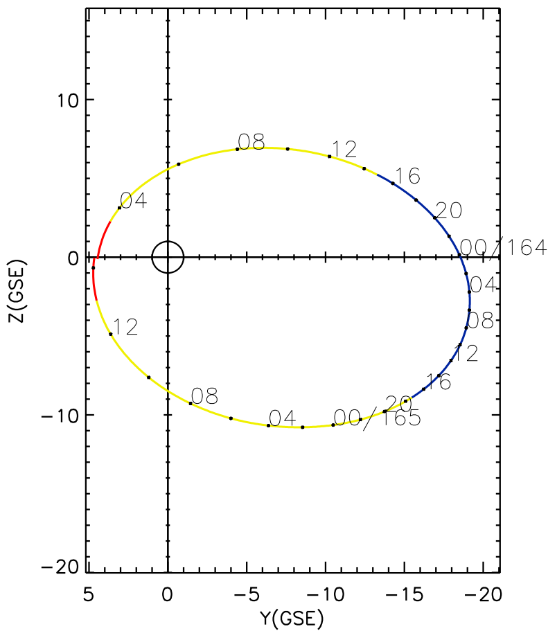
CLUSTER 2 orbit 2005 163 (06/12) 02:36 UT to 2005 165 (06/14) 14:16 UT
