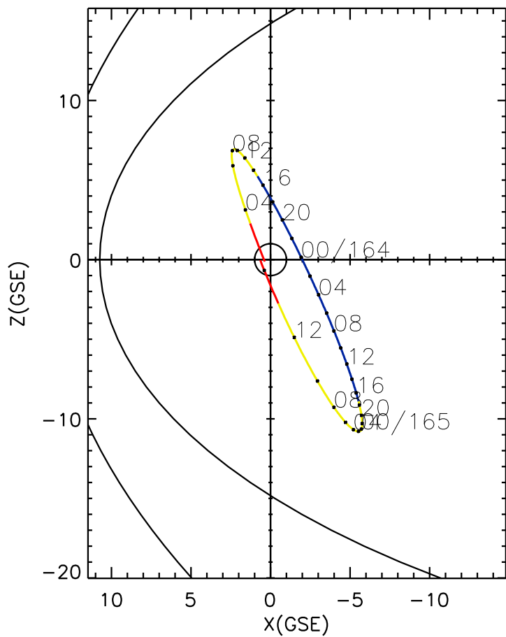
CLUSTER 2 orbit 2005 163 (06/12) 02:36 UT to 2005 165 (06/14) 14:16 UT
