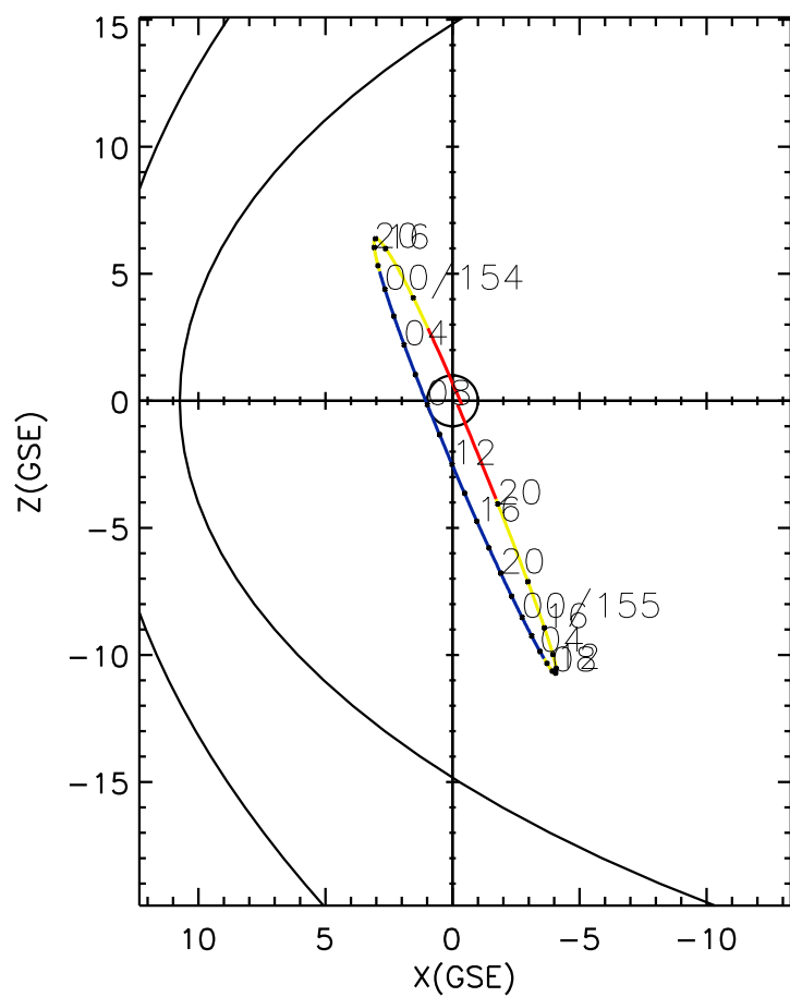
CLUSTER 2 orbit 2005 153 (06/02) 12:06 UT to 2005 155 (06/04) 21:41 UT
