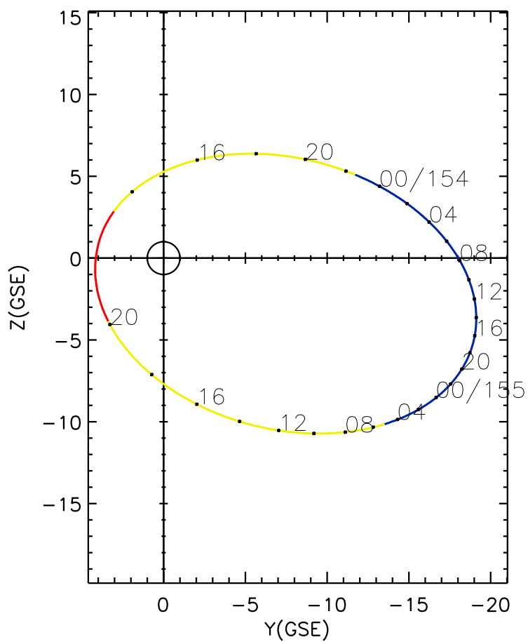
CLUSTER 2 orbit 2005 153 (06/02) 12:06 UT to 2005 155 (06/04) 21:41 UT
