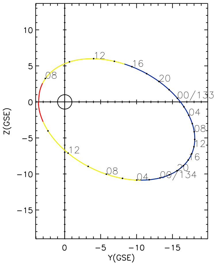
CLUSTER 2 orbit 2005 132 (05/12) 06:36 UT to 2005 134 (05/14) 15:41 UT
