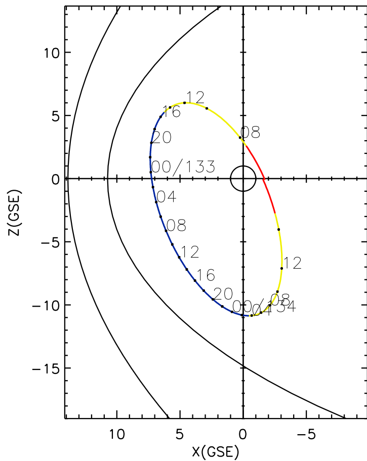
CLUSTER 2 orbit 2005 132 (05/12) 06:36 UT to 2005 134 (05/14) 15:41 UT
