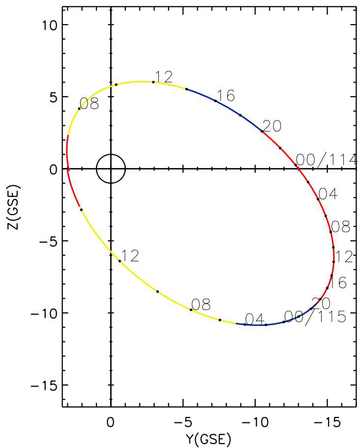
CLUSTER 2 orbit 2005 113 (04/23) 06:01 UT to 2005 115 (04/25) 15:05 UT
