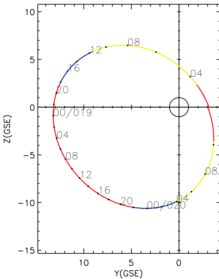
CLUSTER 2 orbit 2005 018 (01/18) 02:36 UT to 2005 020 (01/20) 11:41 UT
