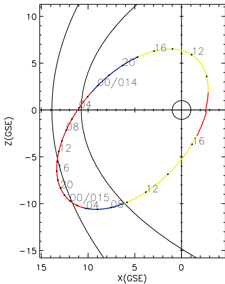
CLUSTER 2 orbit 2005 013 (01/13) 08:21 UT to 2005 015 (01/15) 17:31 UT
