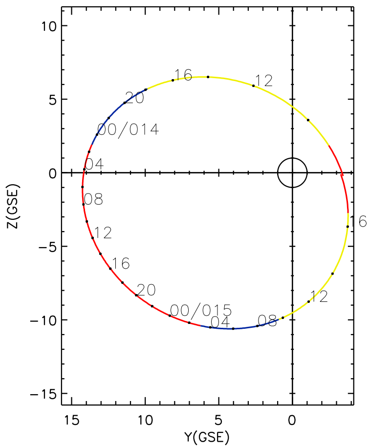
CLUSTER 2 orbit 2005 013 (01/13) 08:21 UT to 2005 015 (01/15) 17:31 UT
