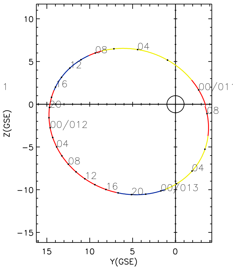
CLUSTER 2 orbit 2005 010 (01/10) 23:16 UT to 2005 013 (01/13) 08:21 UT
