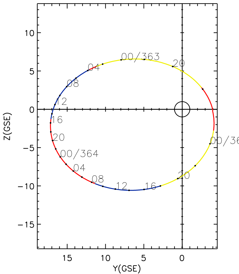
CLUSTER 2 orbit 2004 362 (12/27) 16:51 UT to 2004 365 (12/30) 01:56 UT
