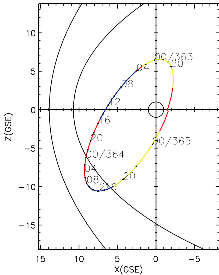
CLUSTER 2 orbit 2004 362 (12/27) 16:51 UT to 2004 365 (12/30) 01:56 UT
