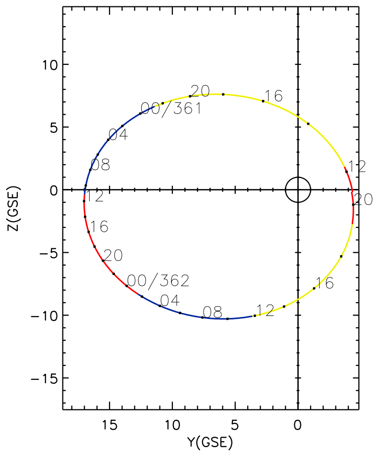
CLUSTER 2 orbit 2004 360 (12/25) 11:20 UT to 2004 362 (12/27) 20:25 UT
