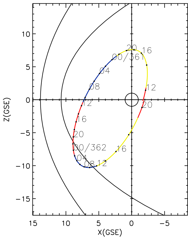
CLUSTER 2 orbit 2004 360 (12/25) 11:20 UT to 2004 362 (12/27) 20:25 UT
