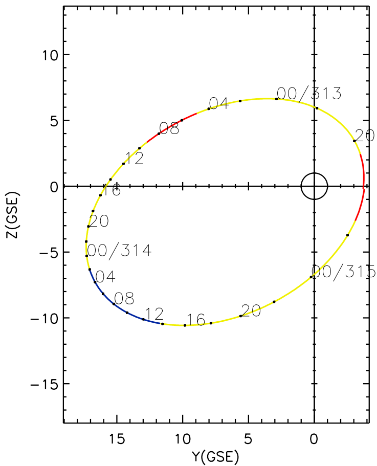
CLUSTER 2 orbit 2004 312 (11/07) 18:26 UT to 2004 315 (11/10) 03:31 UT
