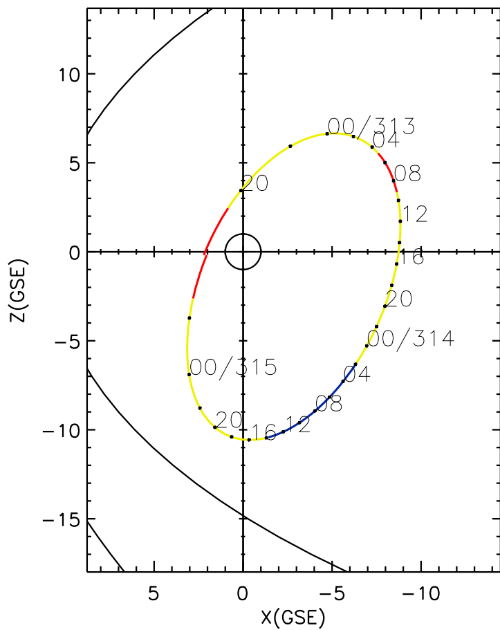
CLUSTER 2 orbit 2004 312 (11/07) 18:26 UT to 2004 315 (11/10) 03:31 UT
