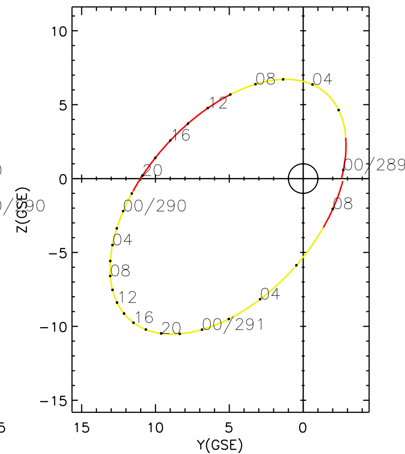
CLUSTER 2 orbit 2004 288 (10/14) 23:46 UT to 2004 291 (10/17) 08:46 UT
