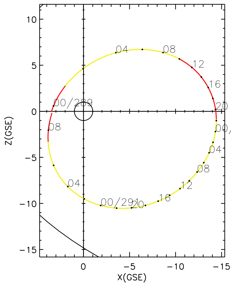
CLUSTER 2 orbit 2004 288 (10/14) 23:46 UT to 2004 291 (10/17) 08:46 UT
