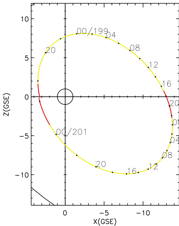
CLUSTER 2 orbit 2004 198 (07/16) 17:05 UT to 2004 201 (07/19) 02:10 UT
