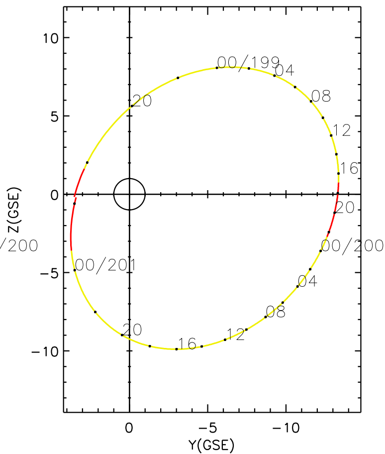
CLUSTER 2 orbit 2004 198 (07/16) 17:05 UT to 2004 201 (07/19) 02:10 UT
