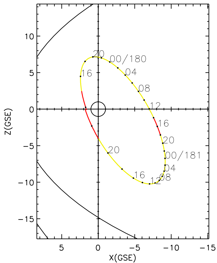
CLUSTER 2 orbit 2004 179 (06/27) 13:51 UT to 2004 181 (06/29) 22:56 UT
