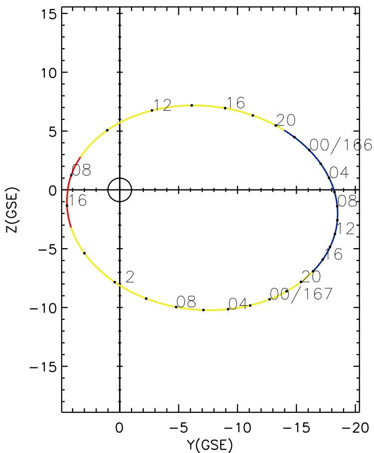
CLUSTER 2 orbit 2004 165 (06/13) 07:26 UT to 2004 167 (06/15) 16:31 UT
