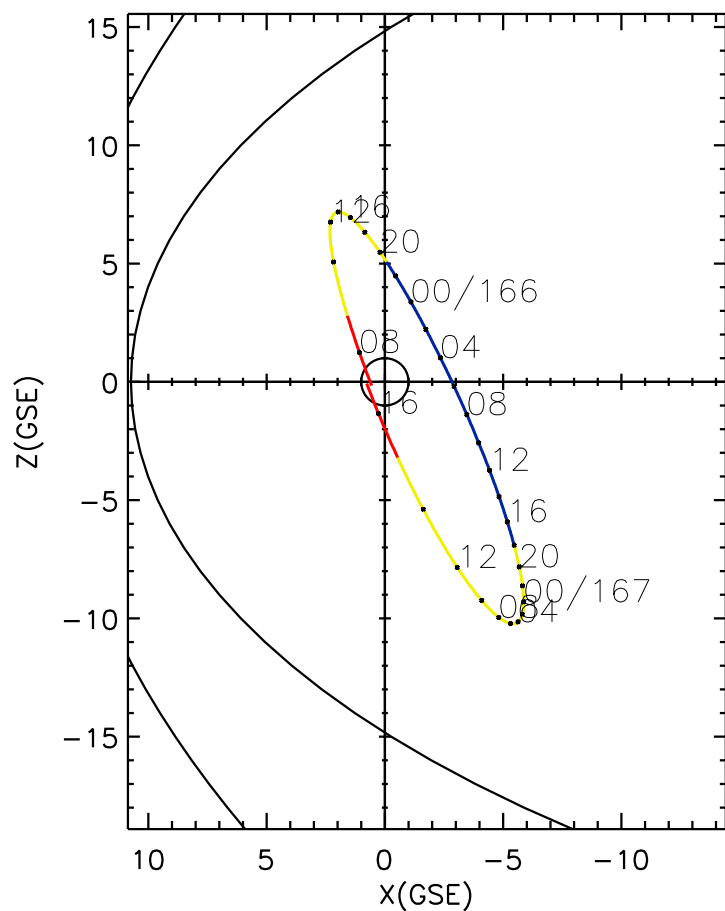
CLUSTER 2 orbit 2004 165 (06/13) 07:26 UT to 2004 167 (06/15) 16:31 UT
