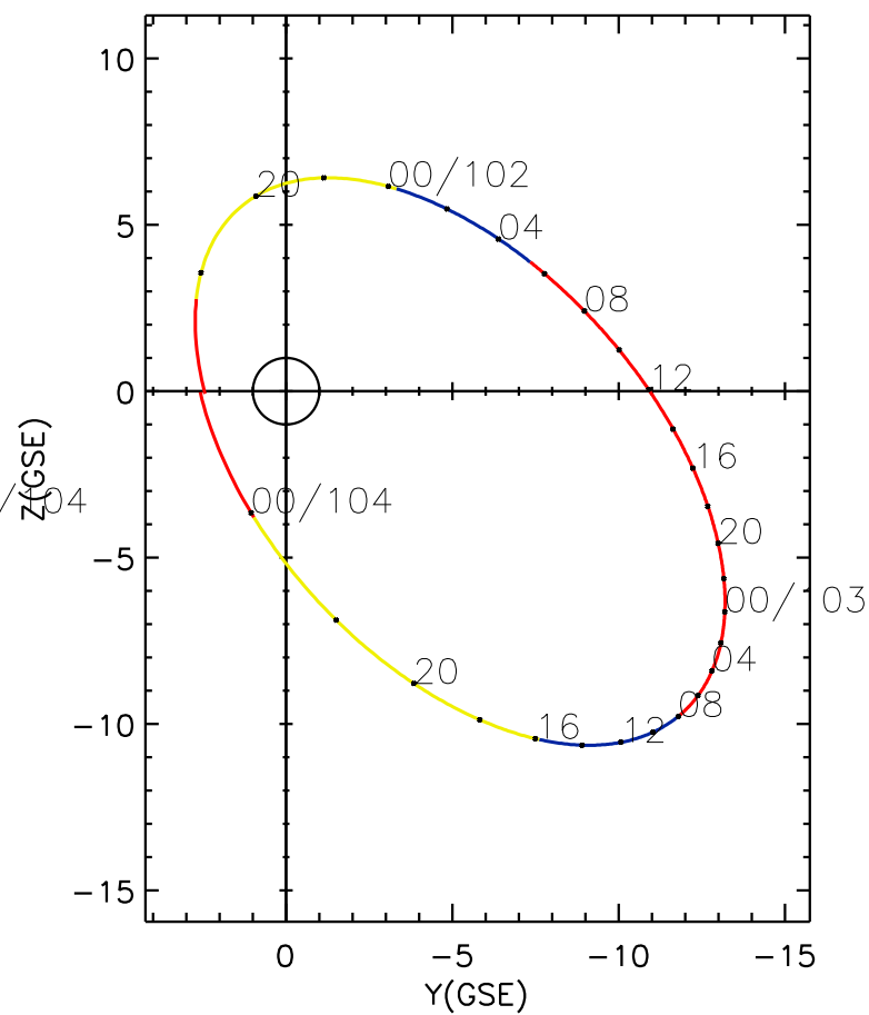
CLUSTER 2 orbit 2004 101 (04/10) 16:26 UT to 2004 104 (04/13) 01:31 UT
