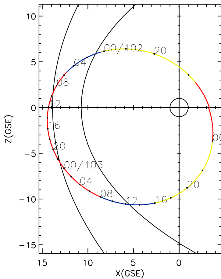
CLUSTER 2 orbit 2004 101 (04/10) 16:26 UT to 2004 104 (04/13) 01:31 UT
