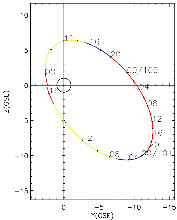
CLUSTER 2 orbit 2004 099 (04/08) 07:20 UT to 2004 101 (04/10) 16:25 UT
