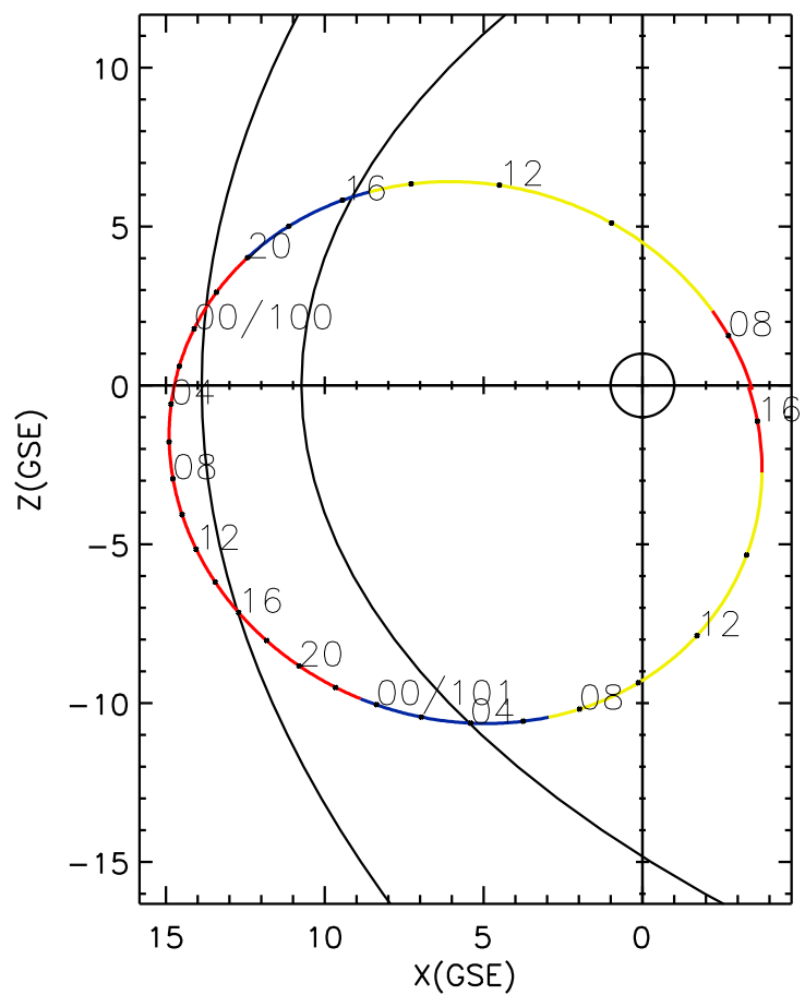
CLUSTER 2 orbit 2004 099 (04/08) 07:20 UT to 2004 101 (04/10) 16:25 UT
