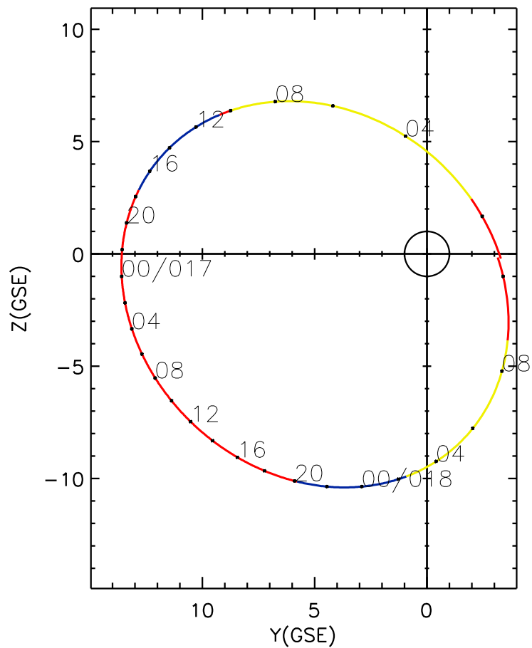
CLUSTER 2 orbit 2004 016 (01/16) 01:15 UT to 2004 018 (01/18) 10:20 UT
