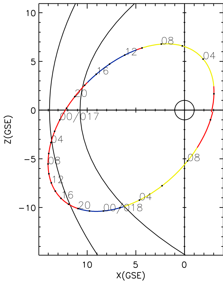
CLUSTER 2 orbit 2004 016 (01/16) 01:15 UT to 2004 018 (01/18) 10:20 UT
