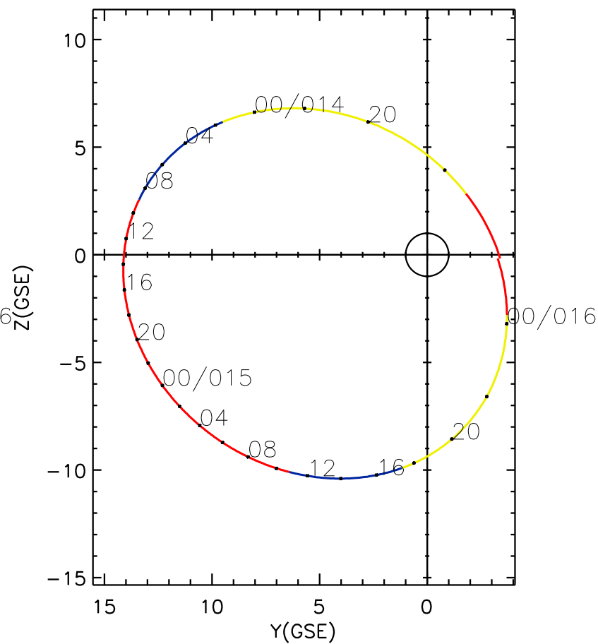
CLUSTER 2 orbit 2004 013 (01/13) 16:11 UT to 2004 016 (01/16) 01:16 UT
