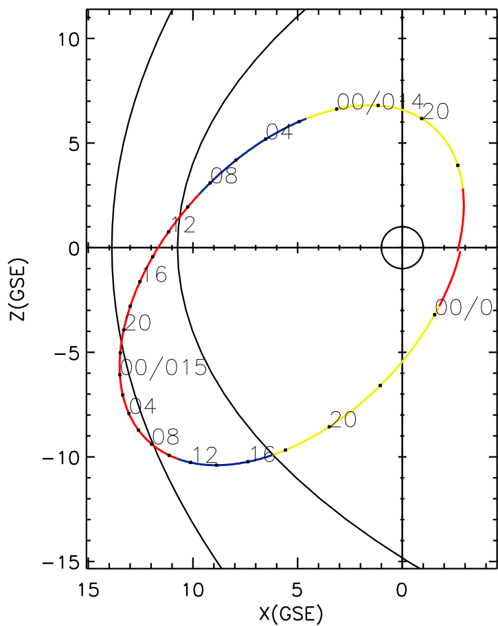
CLUSTER 2 orbit 2004 013 (01/13) 16:11 UT to 2004 016 (01/16) 01:16 UT
