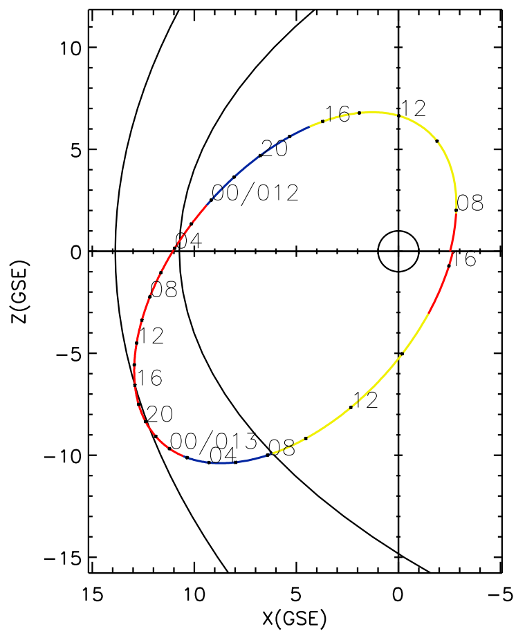
CLUSTER 2 orbit 2004 011 (01/11) 07:11 UT to 2004 013 (01/13) 16:16 UT
