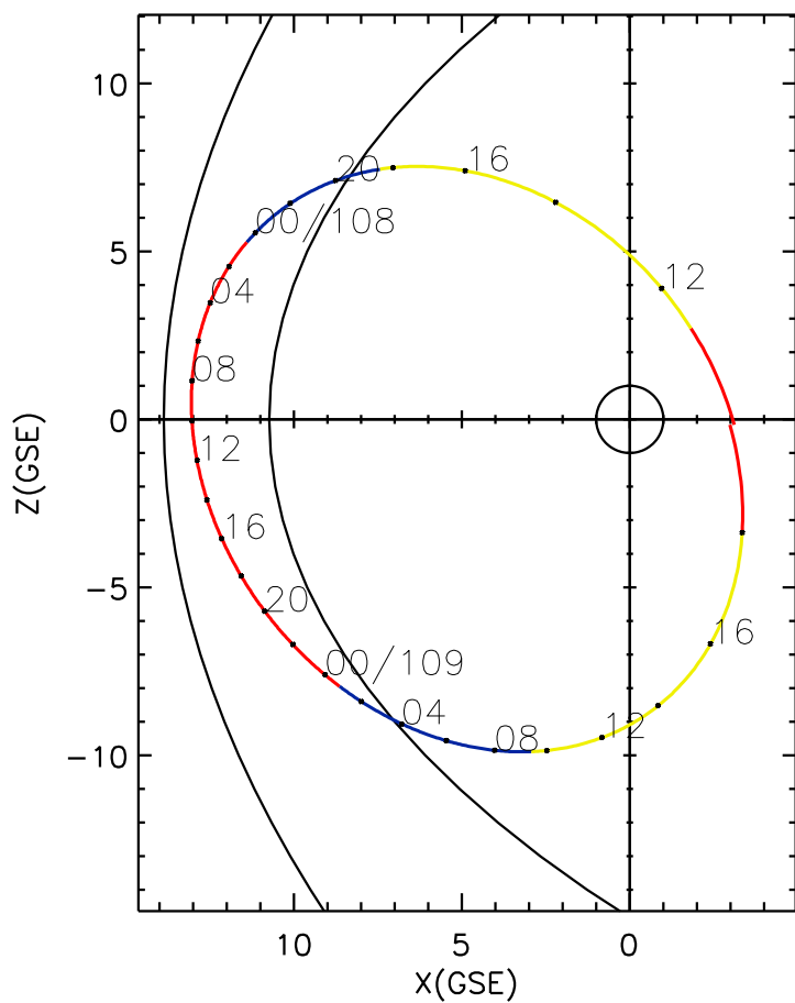
CLUSTER 2 orbit 2003 107 (04/17) 10:15 UT to 2003 109 (04/19) 19:20 UT
