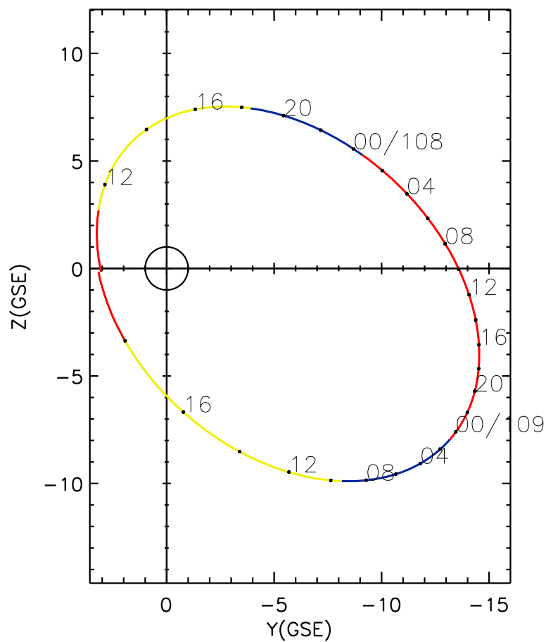
CLUSTER 2 orbit 2003 107 (04/17) 10:15 UT to 2003 109 (04/19) 19:20 UT
