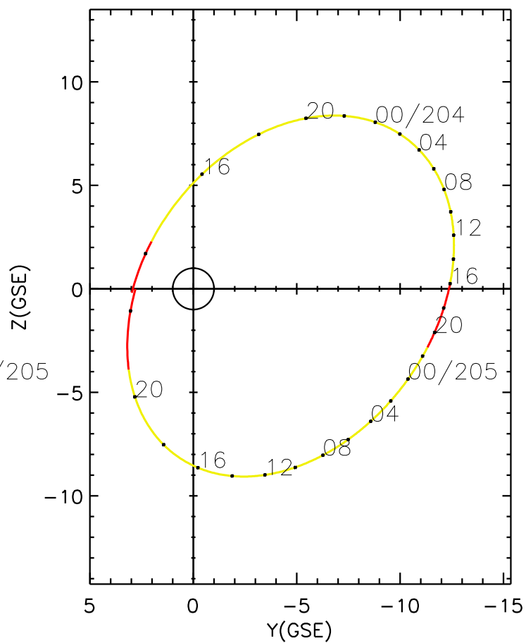
CLUSTER 2 orbit 2002 203 (07/22) 13:15 UT to 2002 205 (07/24) 22:25 UT
