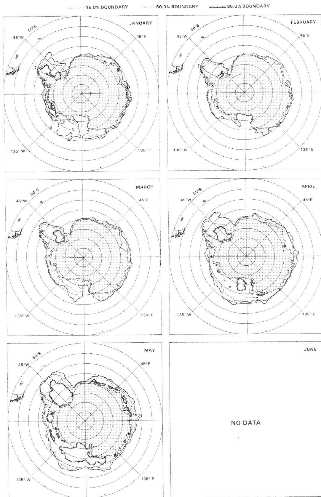
Figure 8. Monthly ice concentration contours for January through June 1975.
