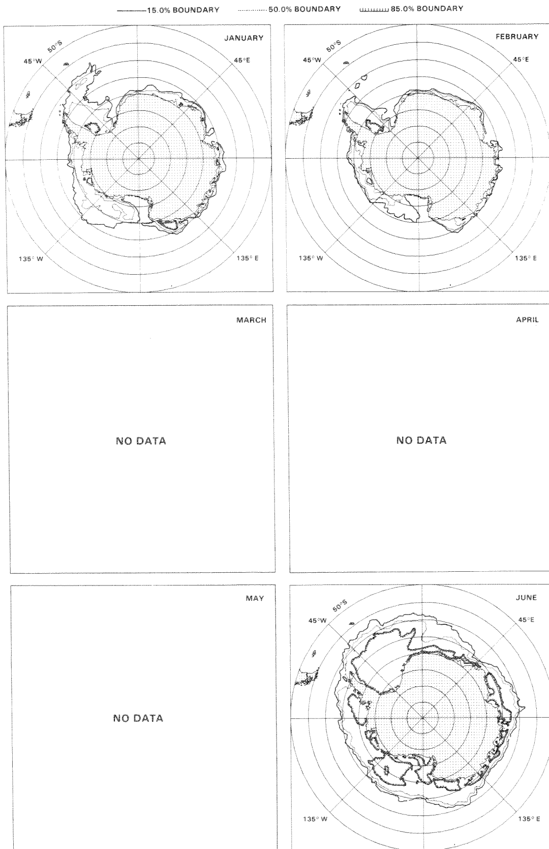
Figure 4. Monthly ice concentration contours for January through June 1973.
