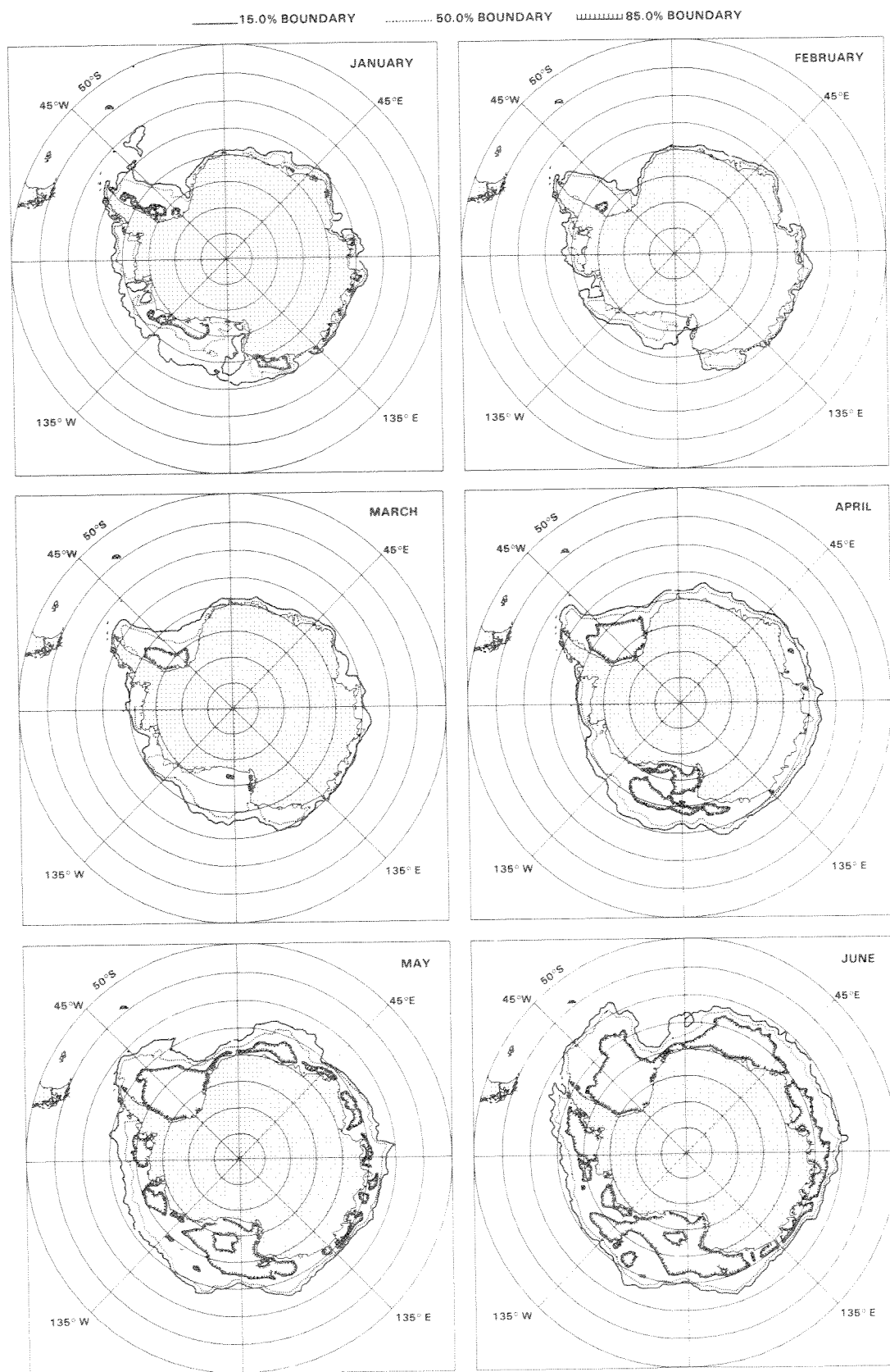
Figure 10. Monthly ice concentration contours for January through June 1976.
