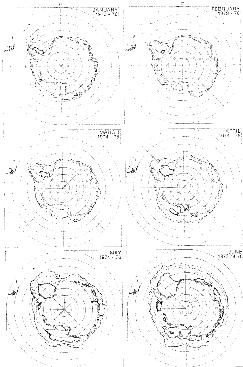
Figure 12. Multiyear monthly ice concentrations contours for January through June 1973-1976.
