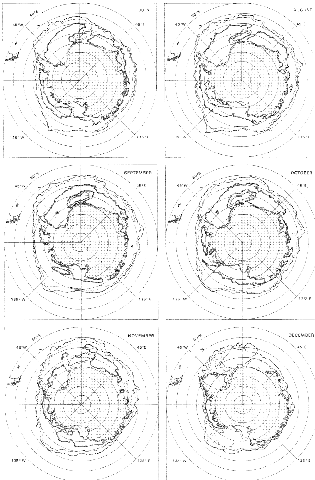
Figure 7. Monthly ice concentration contours for July through December 1974.
