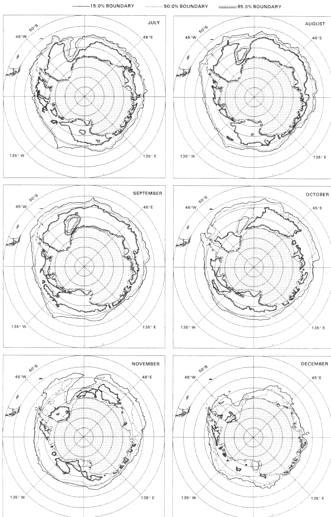
Figure 11. Monthly ice concentration contours for July through December 1976.
