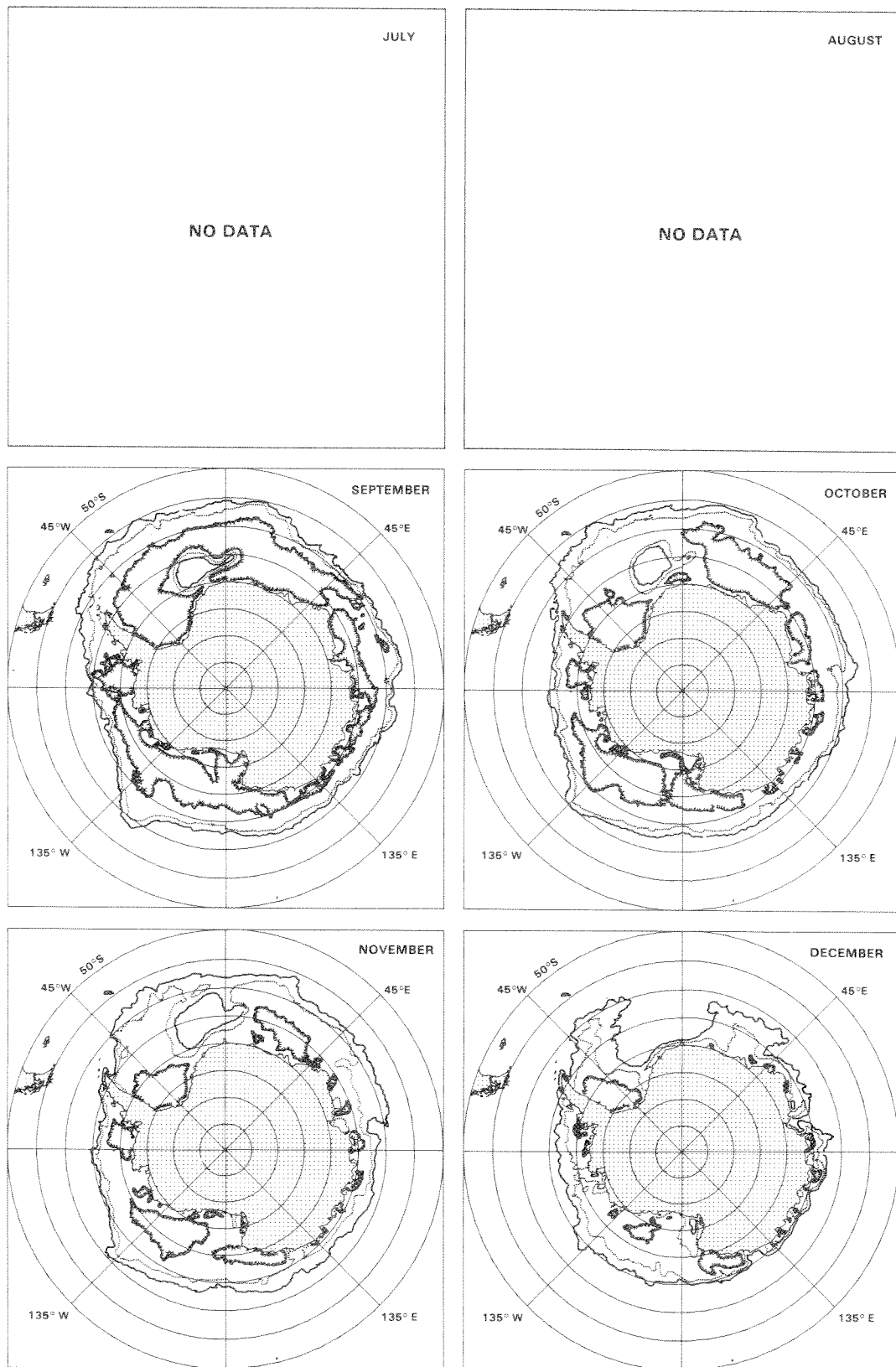
Figure 9. Monthly ice concentration contours for July through December 1975.
