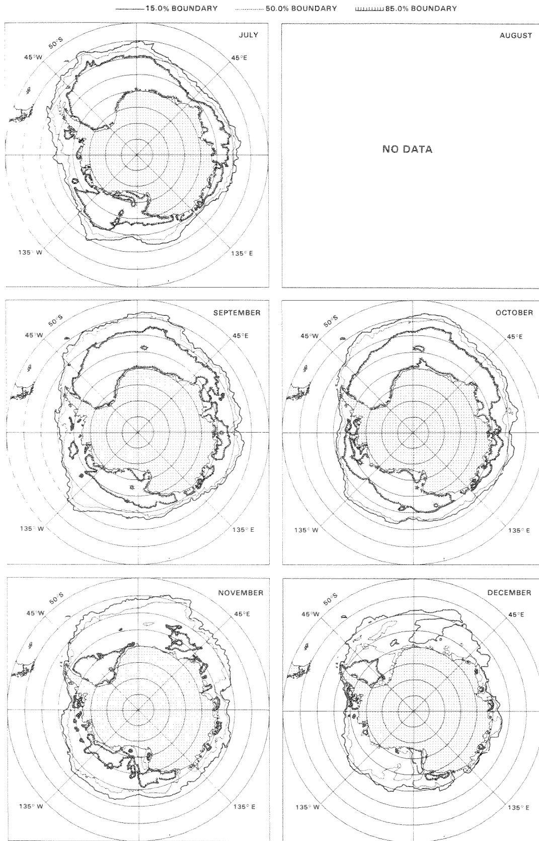
Figure 5. Monthly ice concentration contours for July through December 1973.
