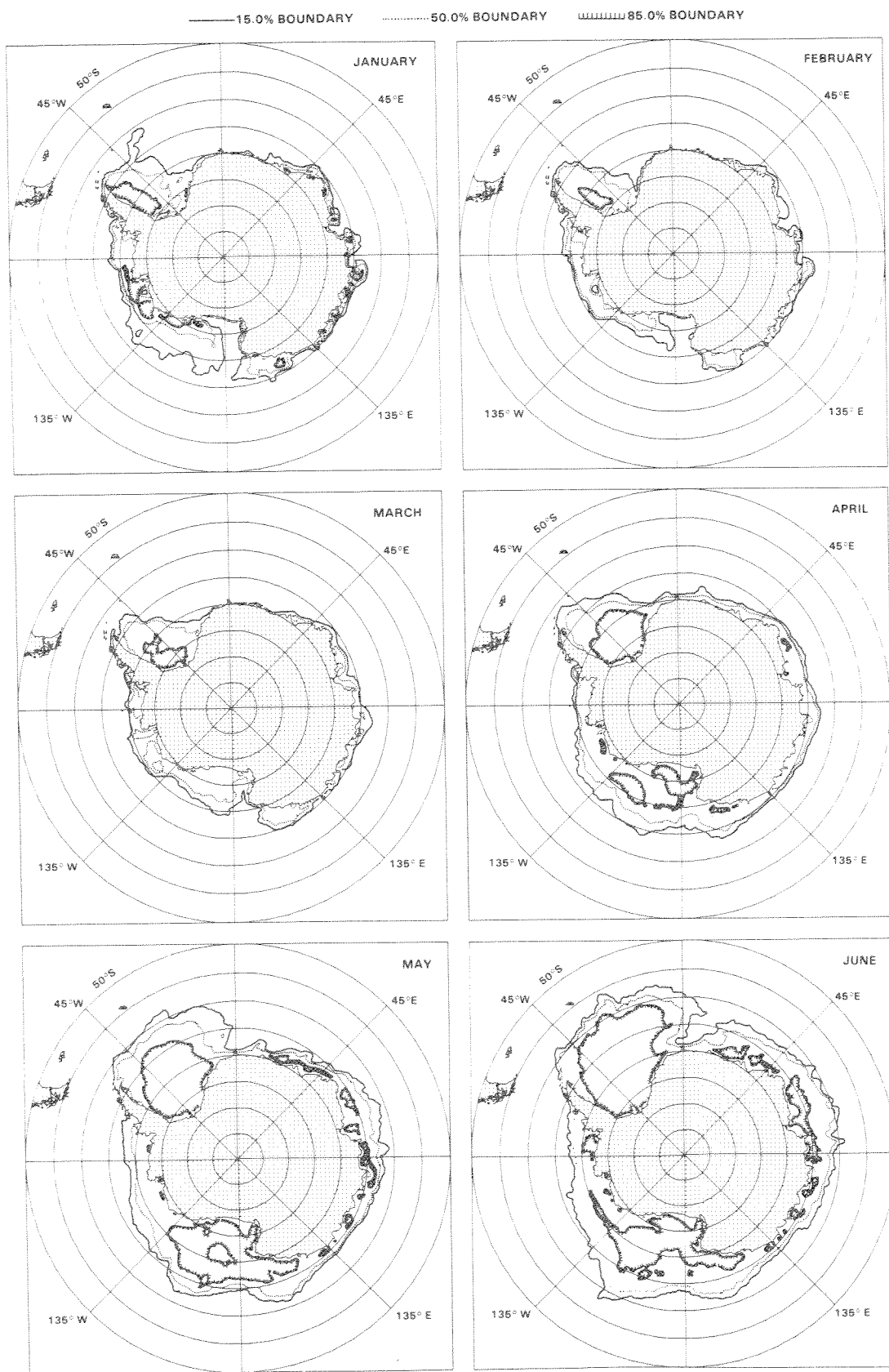
Figure 6. Monthly ice concentration contours for January through June 1974.
