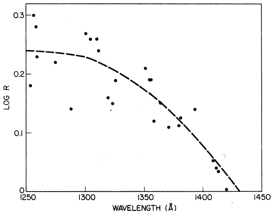
Fig. 4 — Ratio of intensities, reflight instrument, to CALROC.
