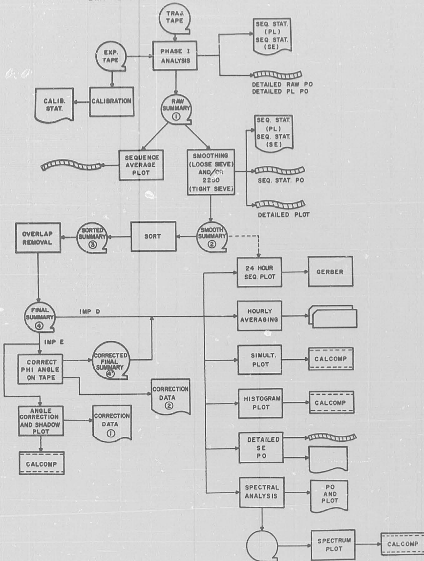
Figure 2. AIMP D and E Data Processing System
