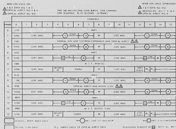
Figure 1. AIMP D (top) and E Encoder Formats
