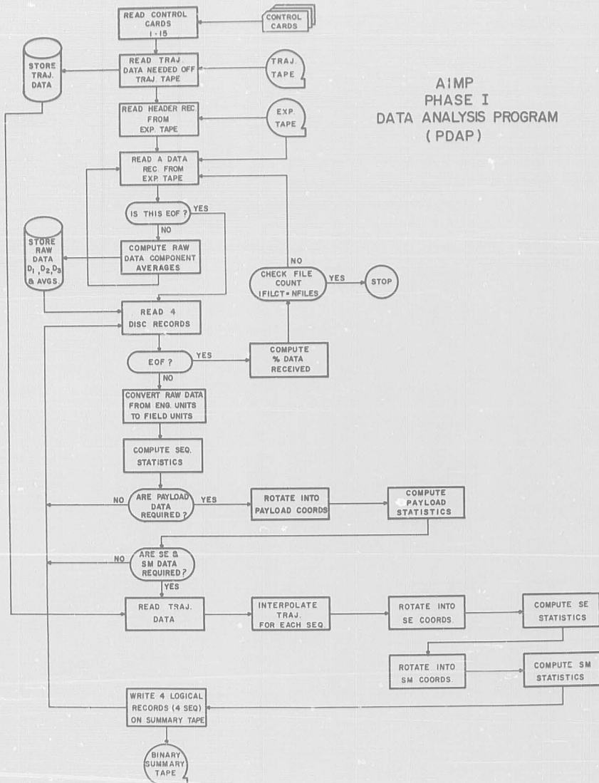
Figure 3. Phase I Analysis Flowchart
