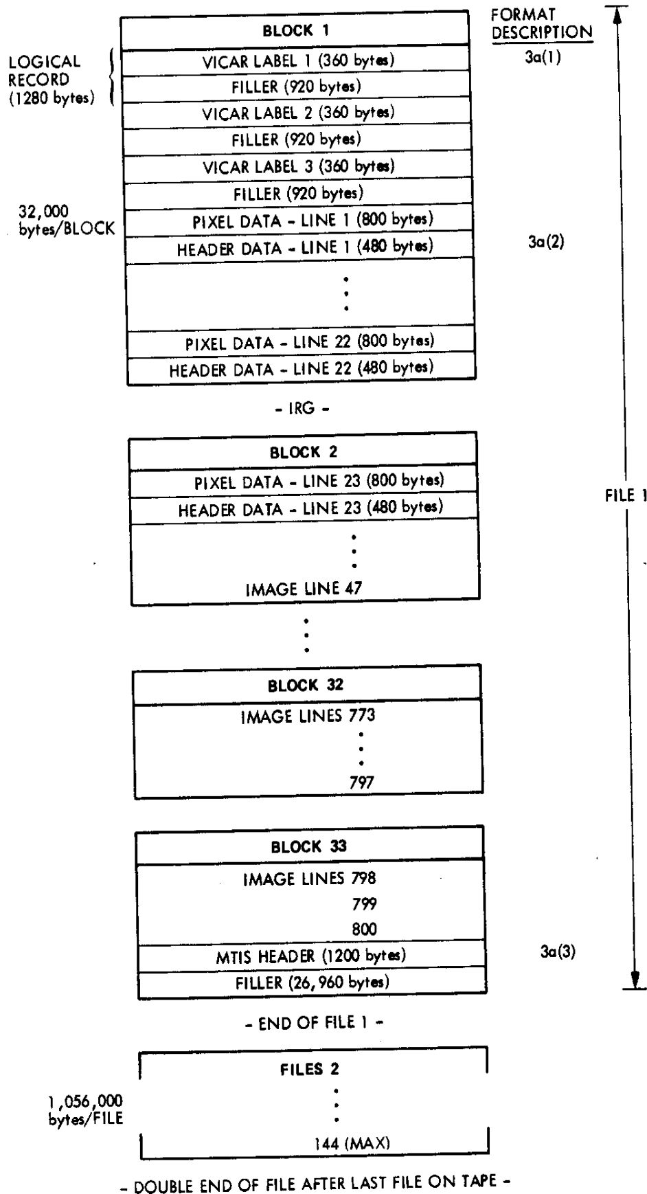
Figure A-1. Voyager Image File Format
