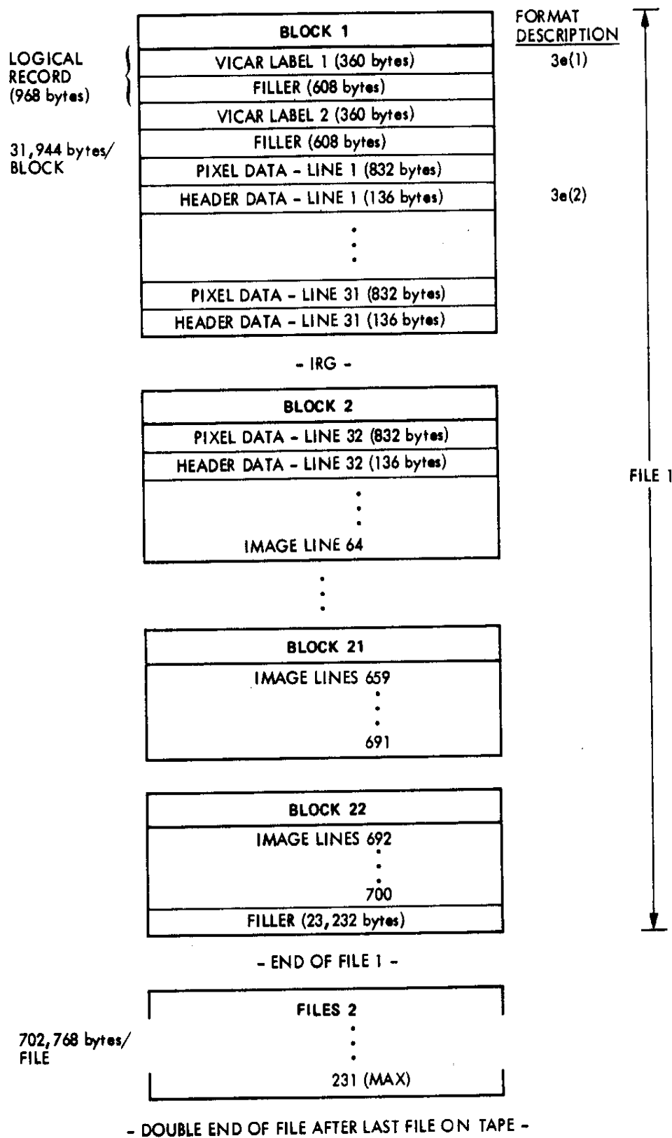
Figure A-5. Mariner 9 Image File Format
