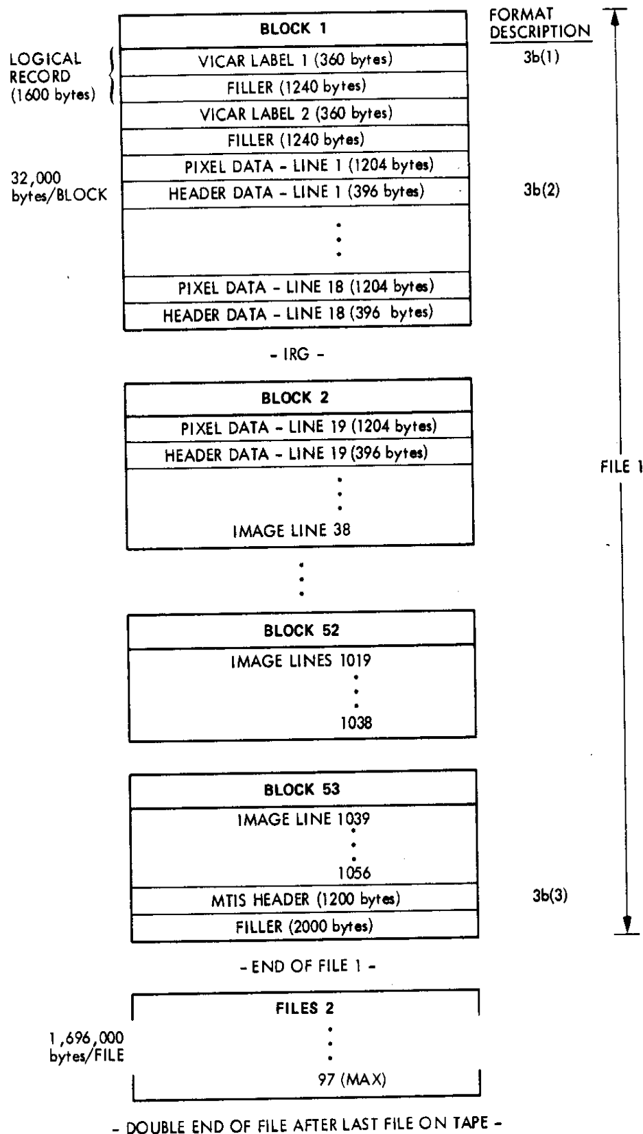
Figure A-2. Viking Orbiter Image File Format
