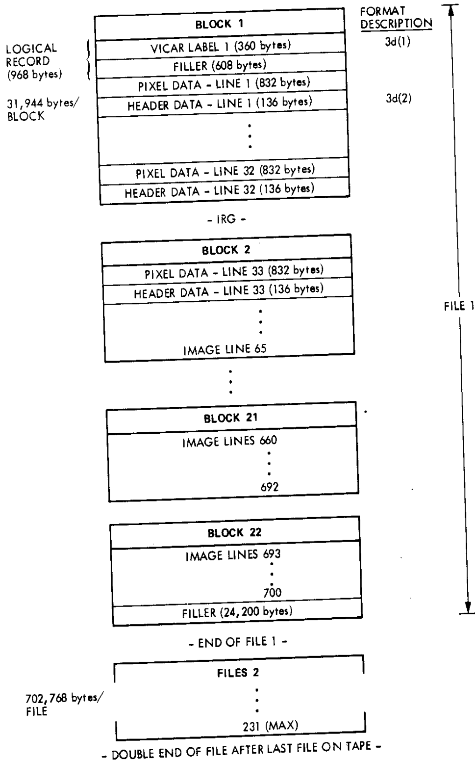
Figure A-4. Mariner 10 Image File Format
