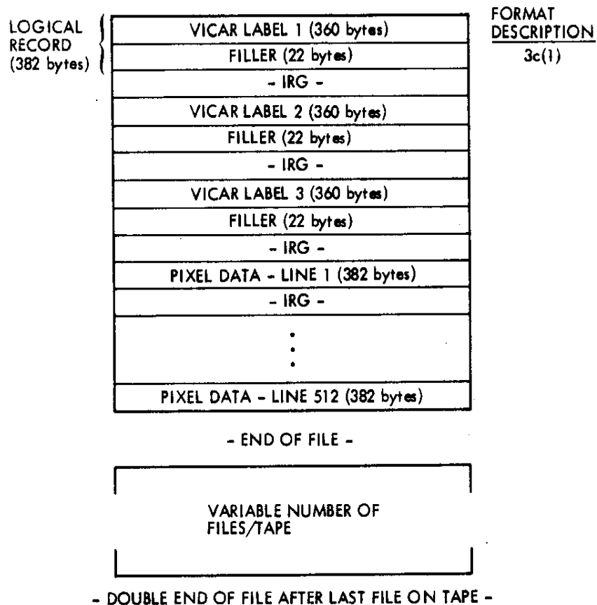
Figure A-3. Viking Lander Image File Format
