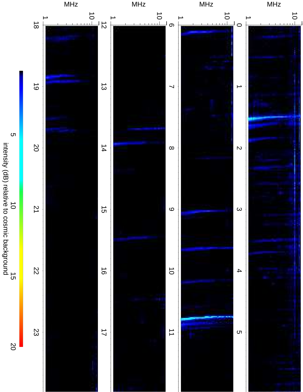
Wind Waves RAD2 receiver: 2021/10/04
