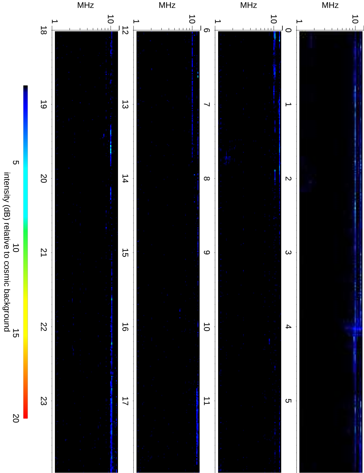
Wind Waves RAD2 receiver: 2020/10/11
