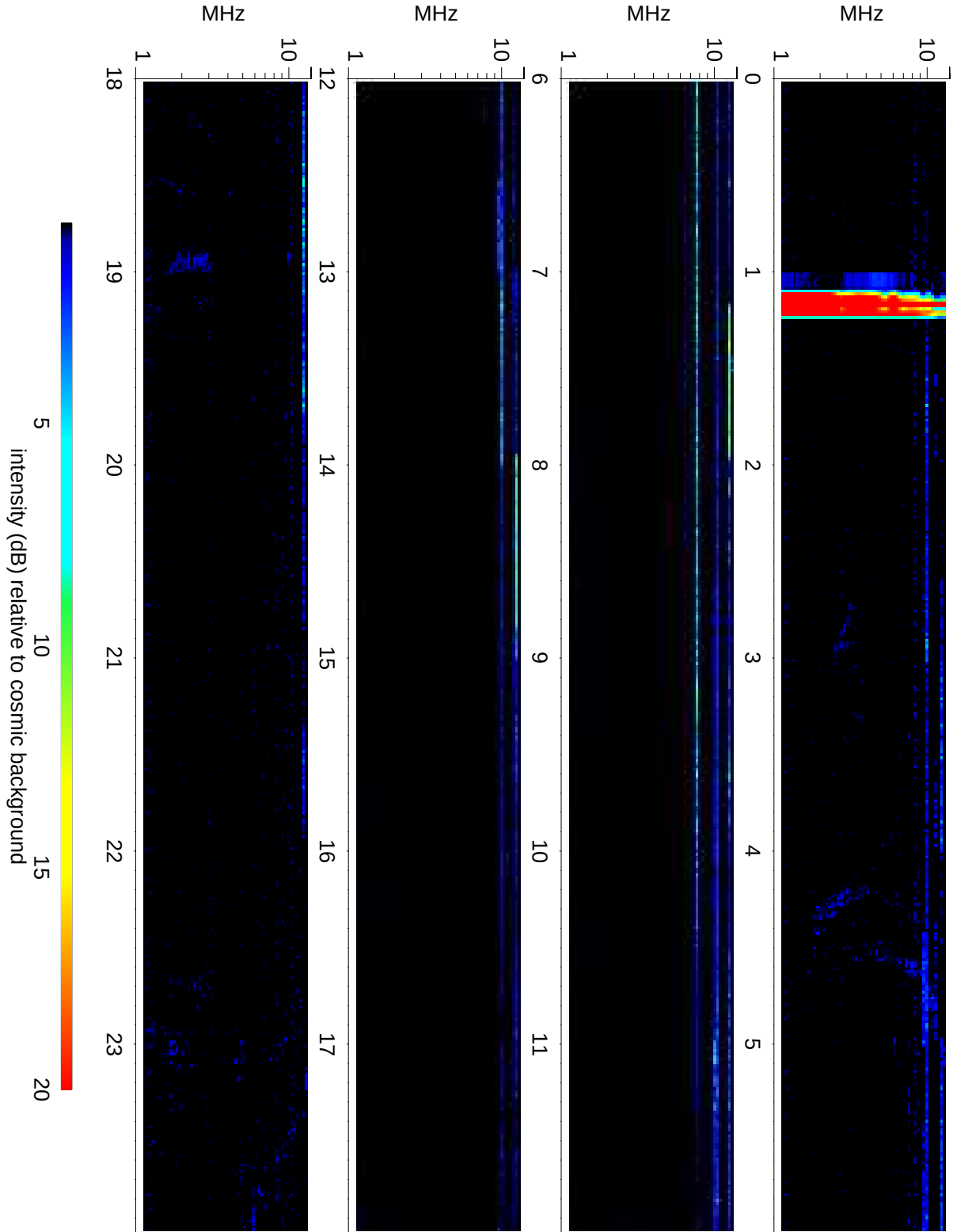
Wind Waves RAD2 receiver: 2020/07/12
