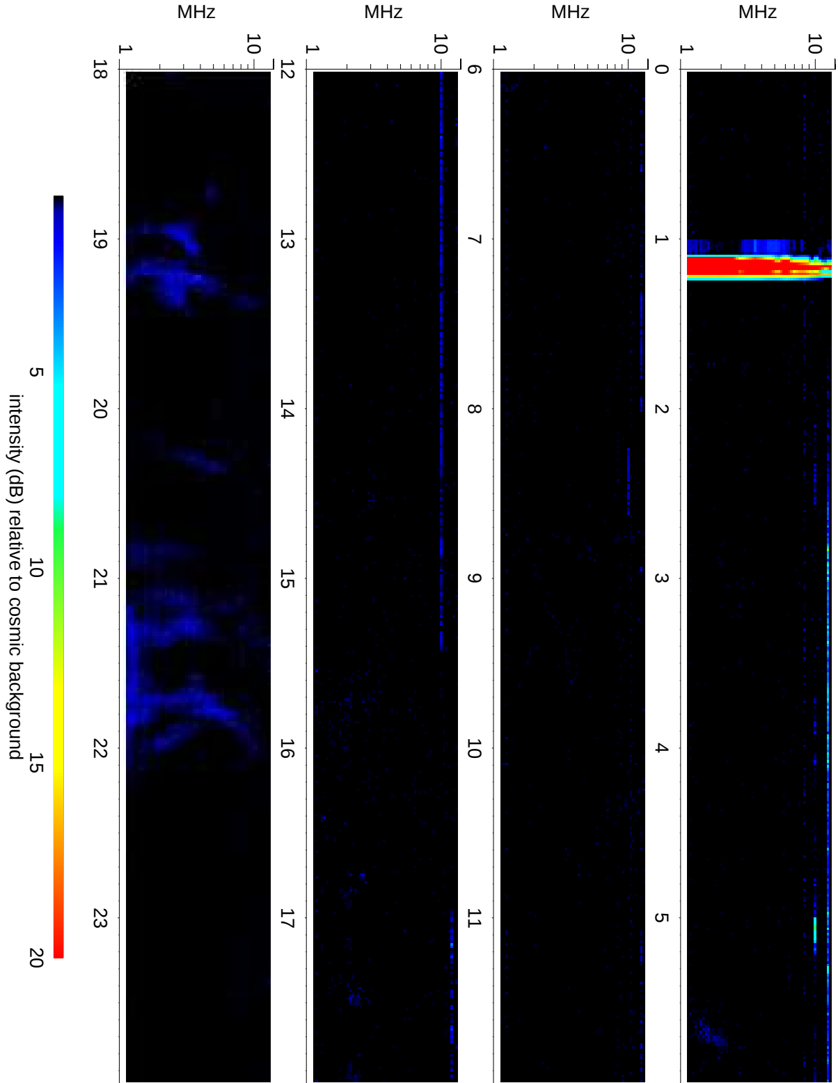
Wind Waves RAD2 receiver: 2019/11/26
