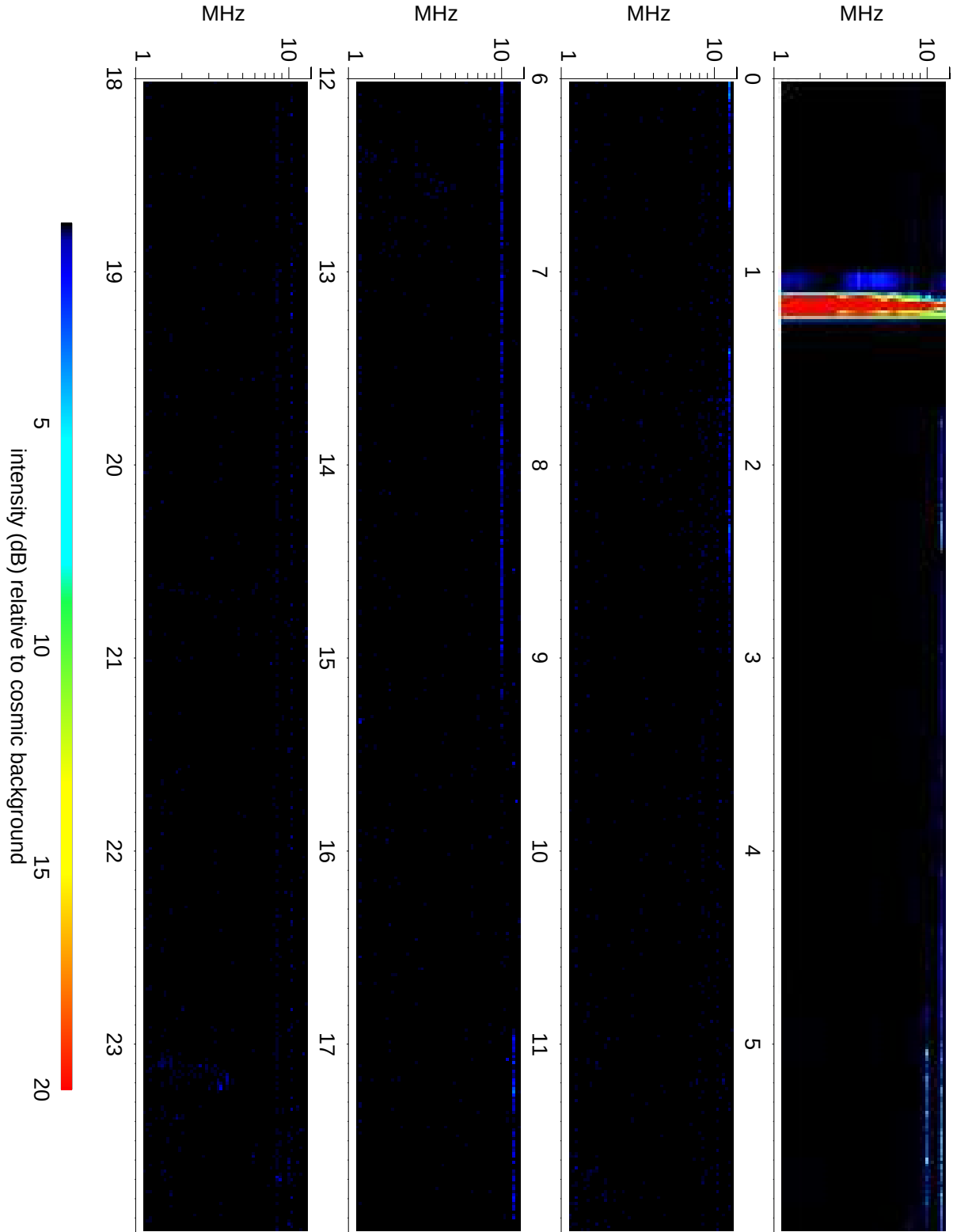
Wind Waves RAD2 receiver: 2019/11/22
