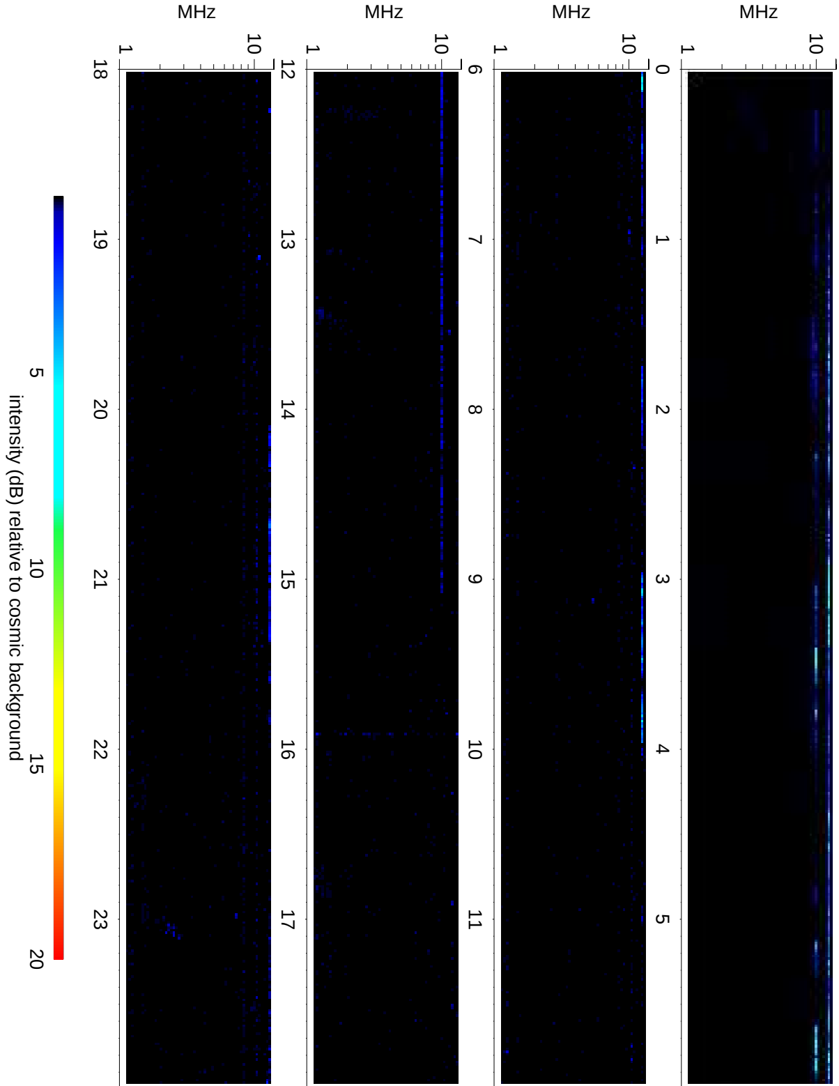
Wind Waves RAD2 receiver: 2019/11/17
