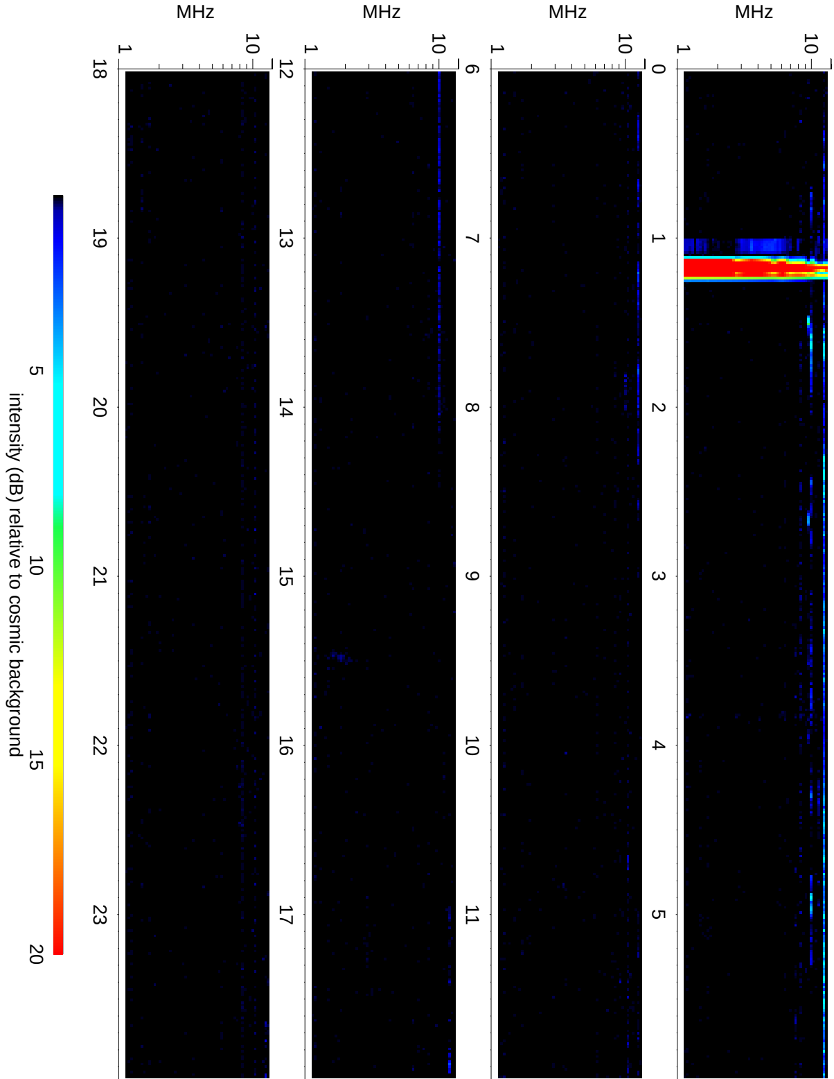
Wind Waves RAD2 receiver: 2019/11/14
